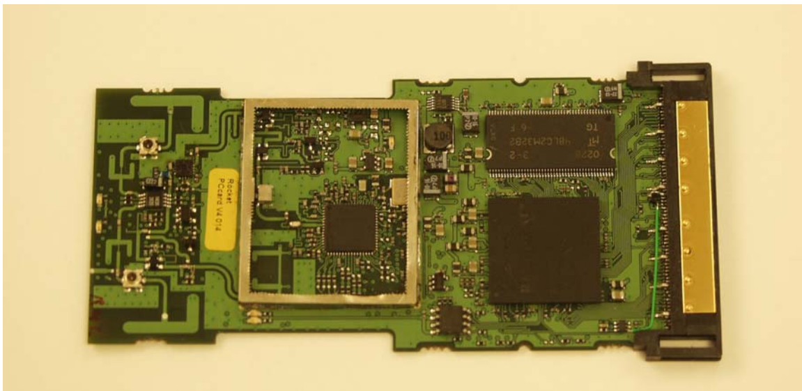
Top of Card (shield removed)
