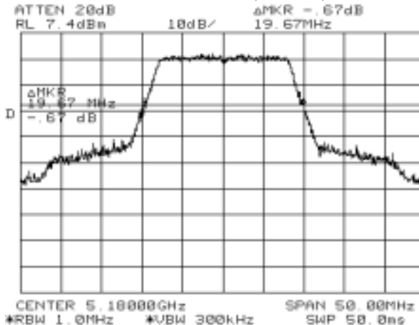
301(20dB BW)
