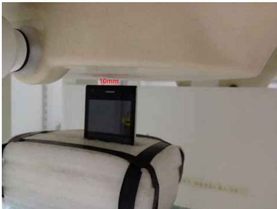
Body SAR Top Side 10mm for WLAN
