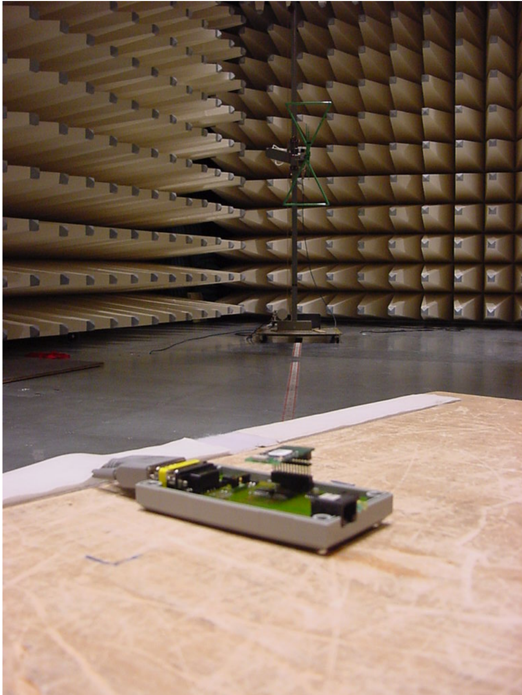
Photo 1: Radiated Emissions
