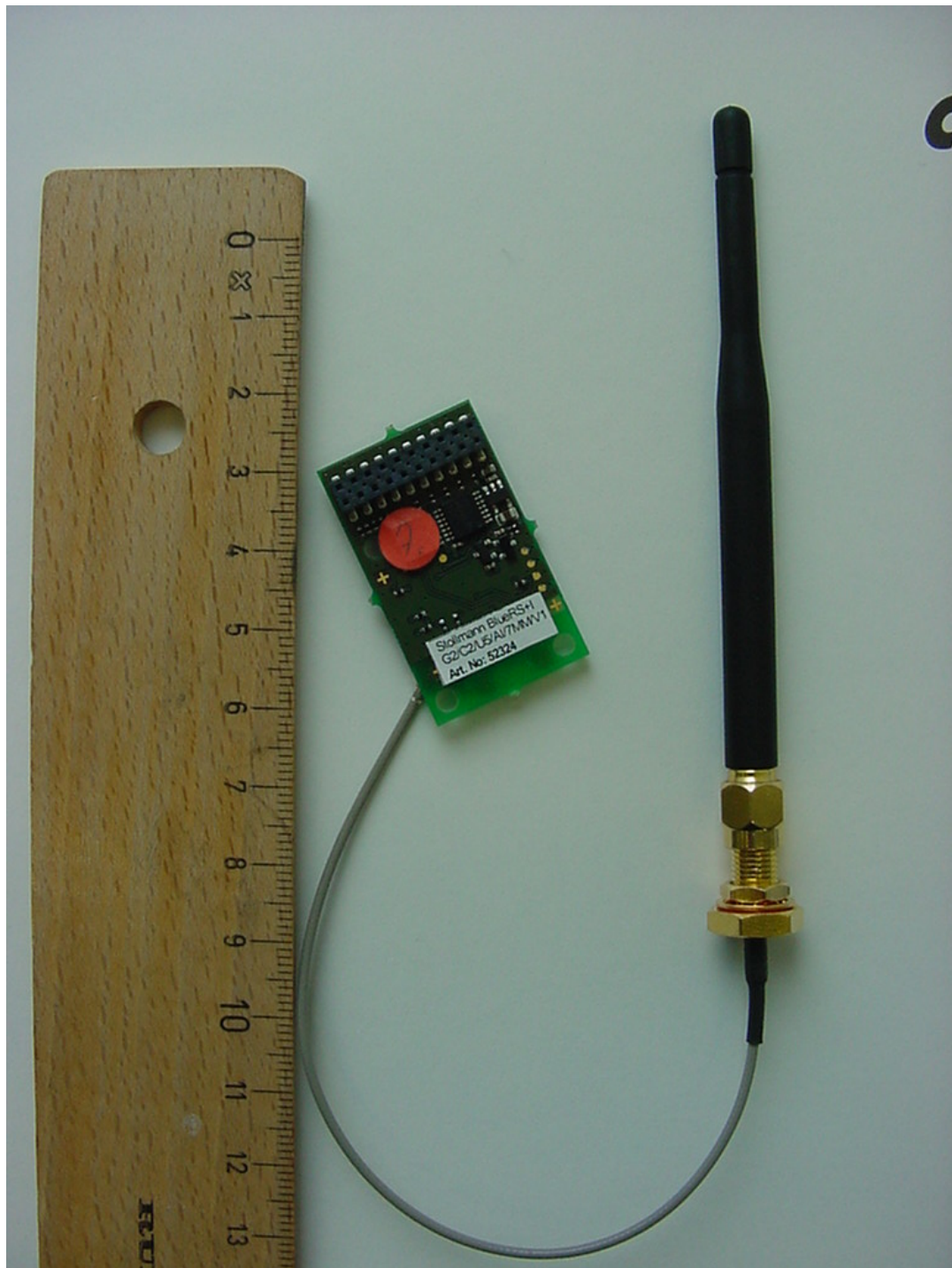
Photo 1: with external antenna
