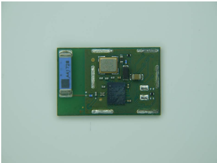
Photo 1: Module without shielding, PMN: BlueMod+S50/AI
