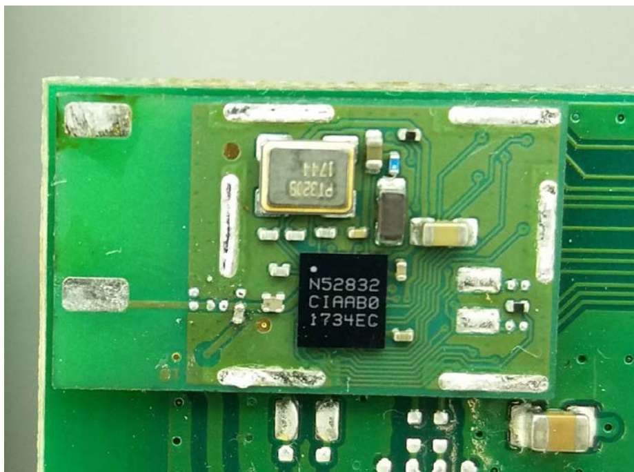
Photo 2: Module without shielding, PMN: BlueMod+S50/AP
