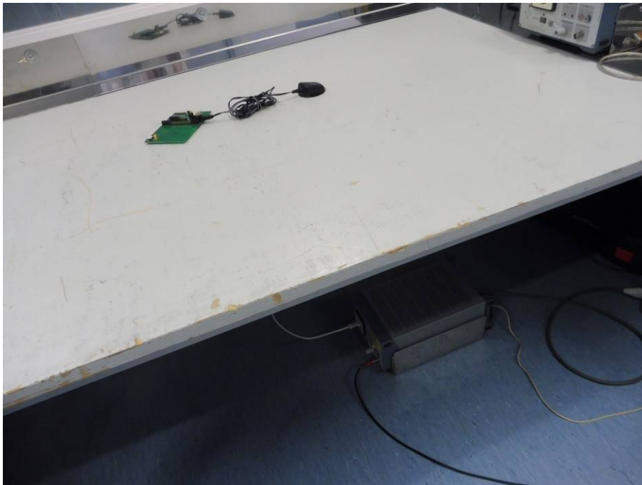
Photo 8: module with on-board antenna
