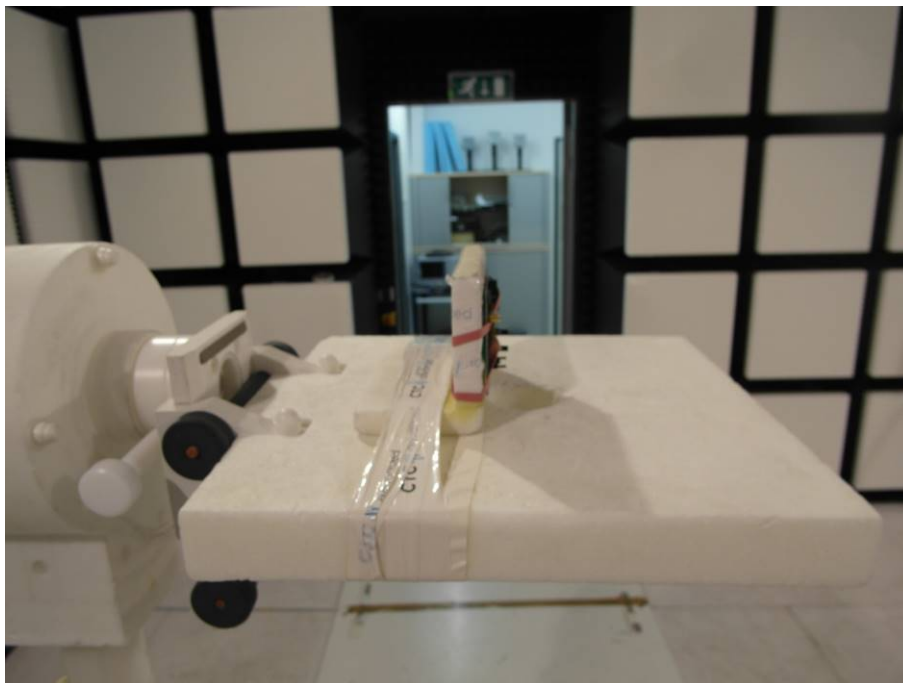
Photo 3: module with on-board antenna
