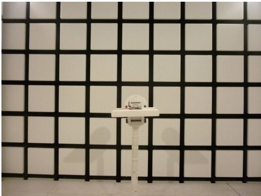
Photo 12: module with external antenna on eval board
