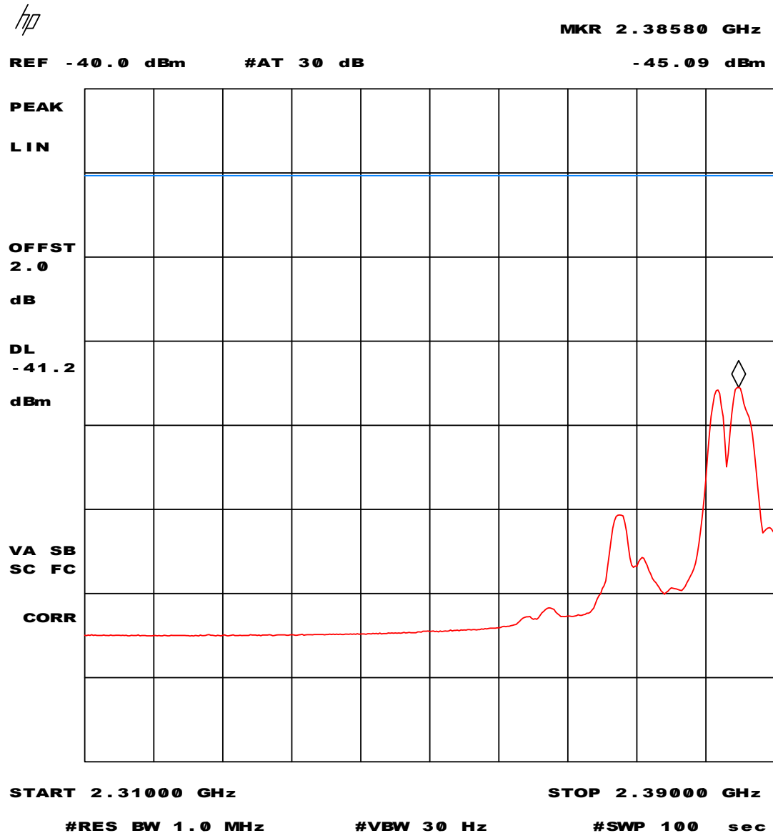
Plot 1 - Average measurement values in restricted band 2310 - 2390 MHz.
