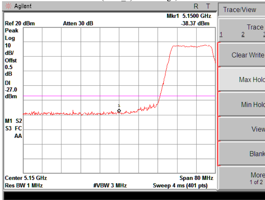
TX Mode (ANT_3): Band Edge, Left Side
