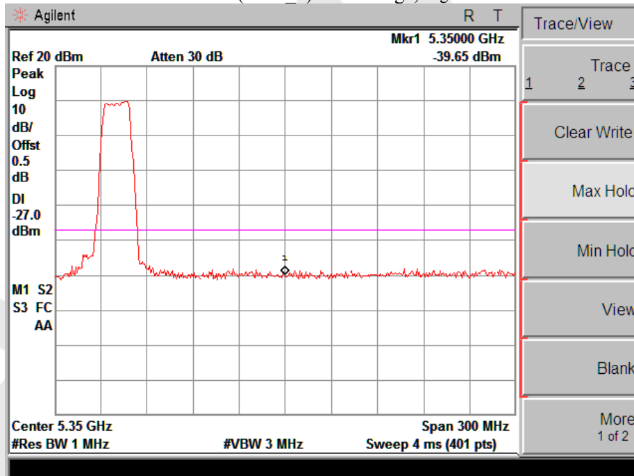
TX Mode (ANT_4): Band Edge, Right Side
