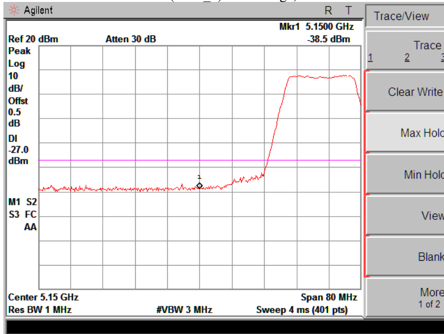
TX Mode (ANT_2): Band Edge, Left Side
