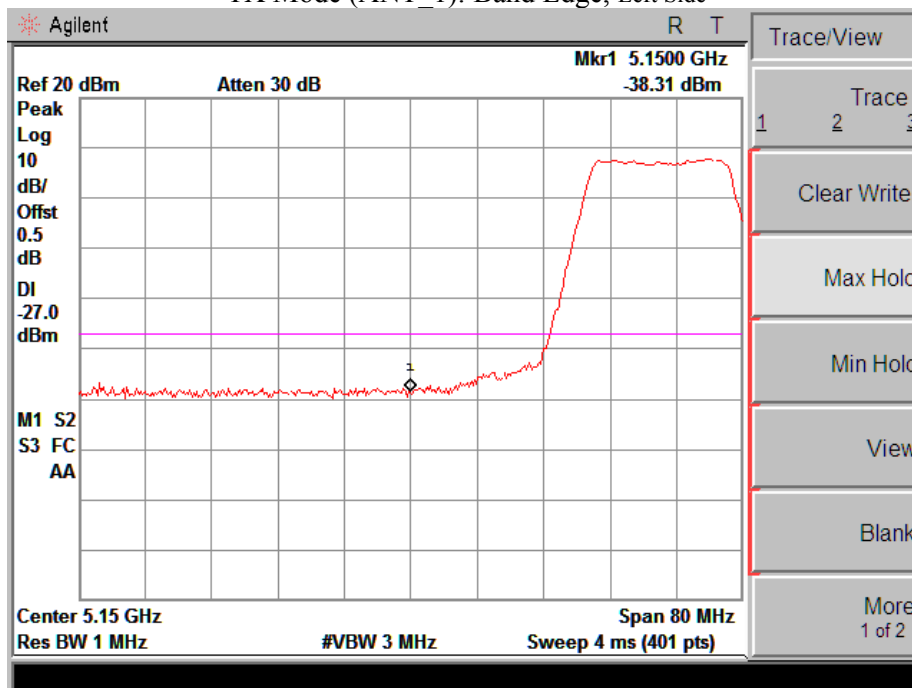
TX Mode (ANT_1): Band Edge, Left Side
