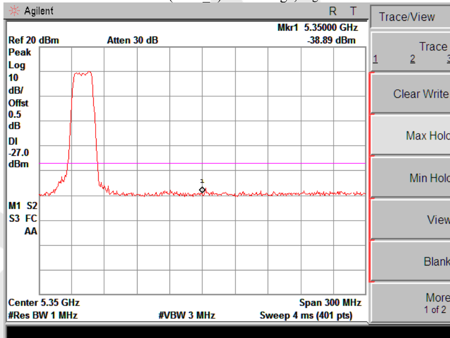
TX Mode (ANT_3): Band Edge, Right Side
