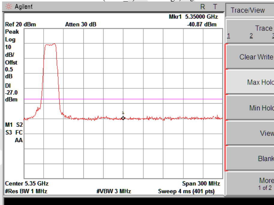
TX Mode (ANT_2): Band Edge, Right Side
