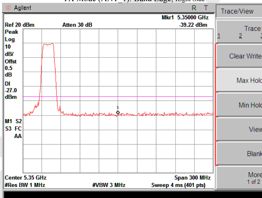
TX Mode (ANT_1): Band Edge, Right Side
