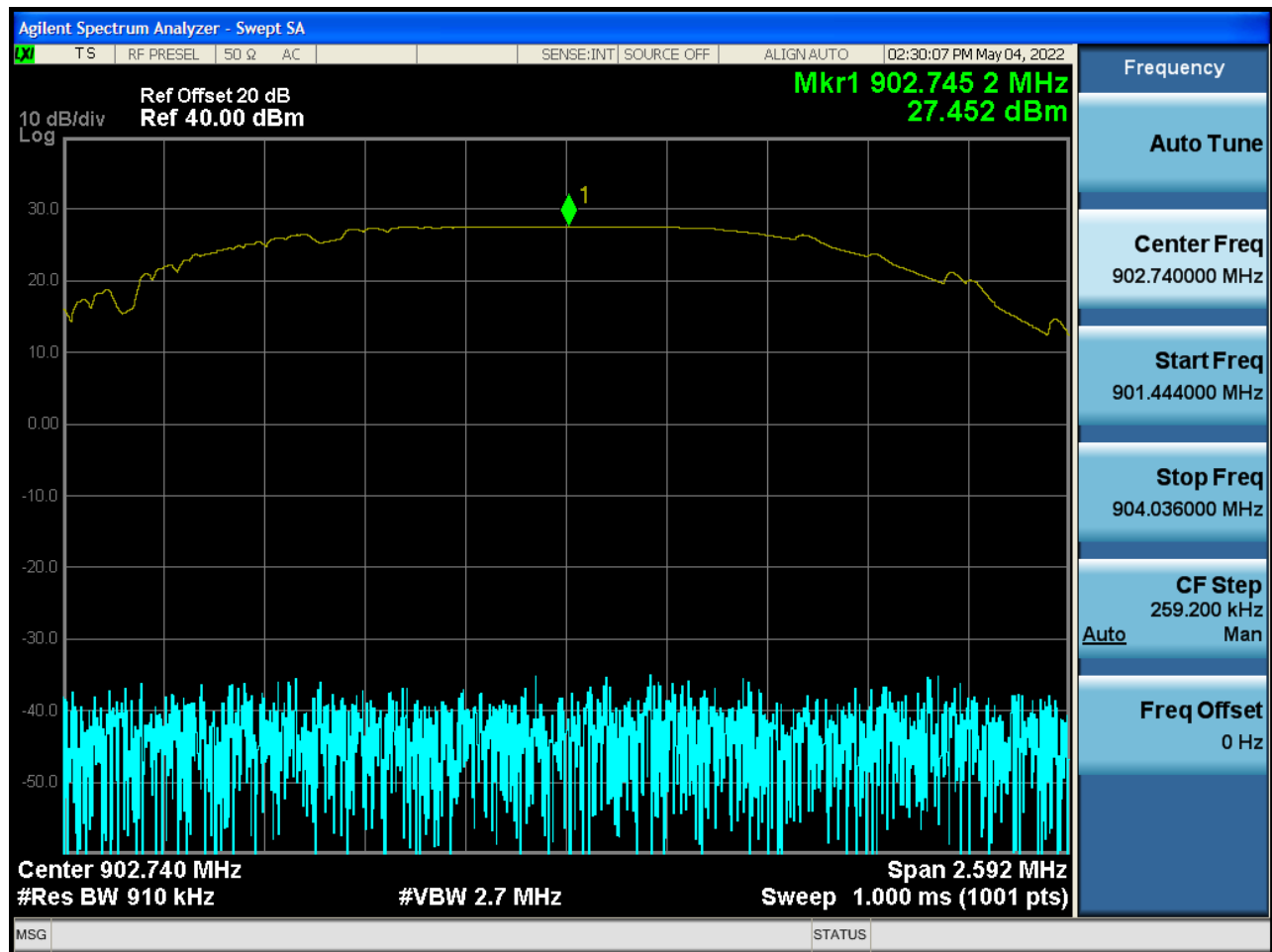
Peak Output Power – Low Channel
