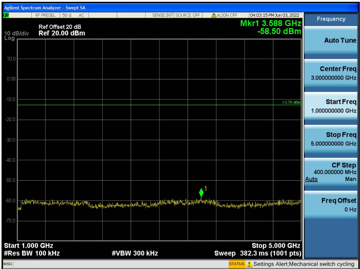
RF Antenna Conducted Test – Mid Channel – 1 GHz to 5 GHz
