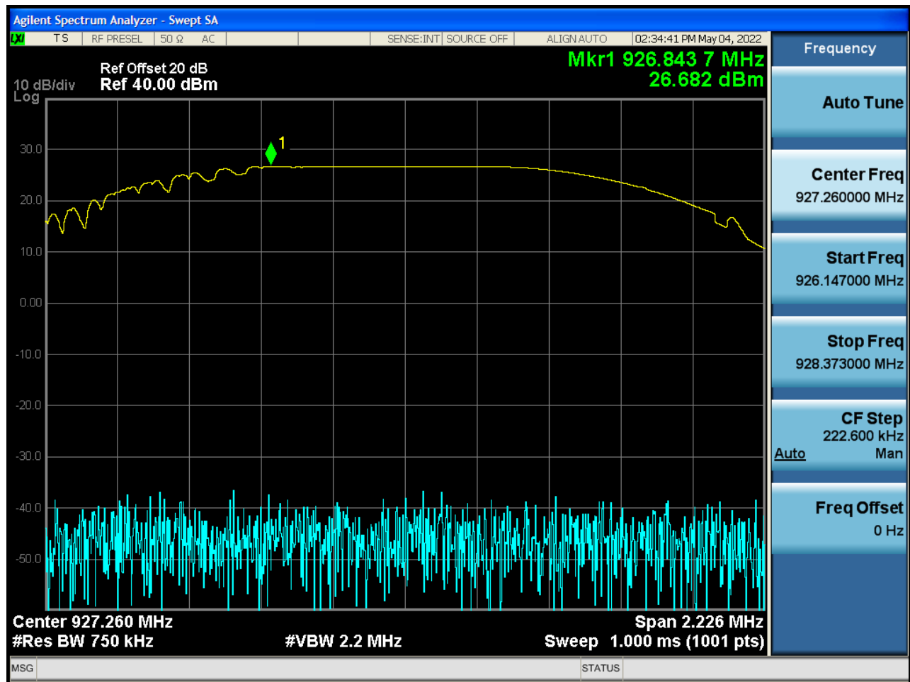
Peak Output Power – High Channel
