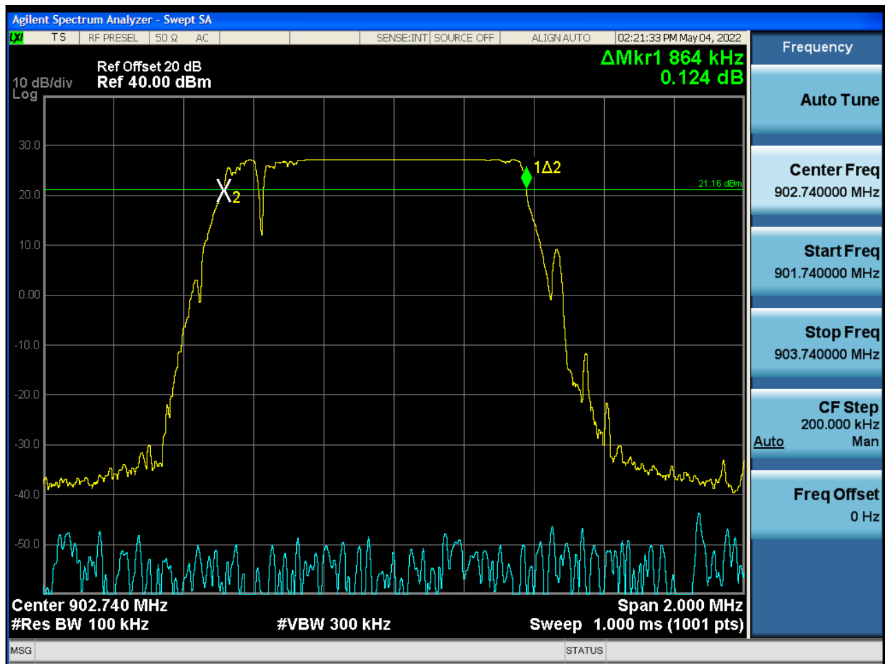
DTS Bandwidth – Low Channel
