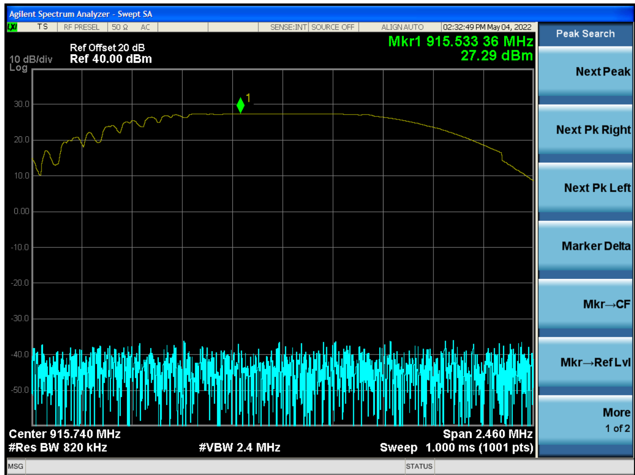
Peak Output Power – Middle Channel
