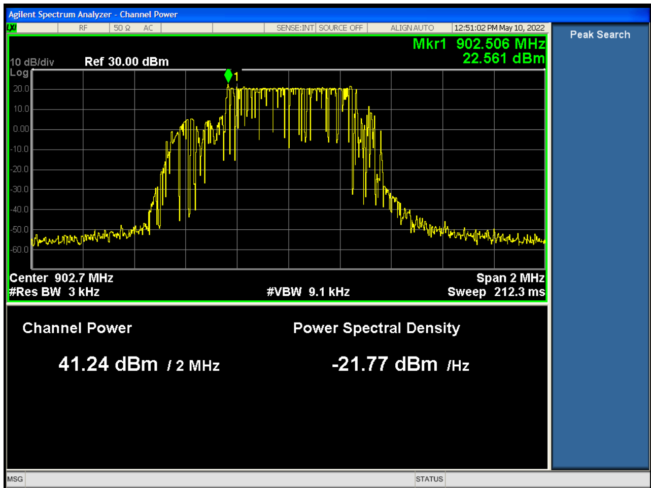
Power Spectral Density – Low Channel
