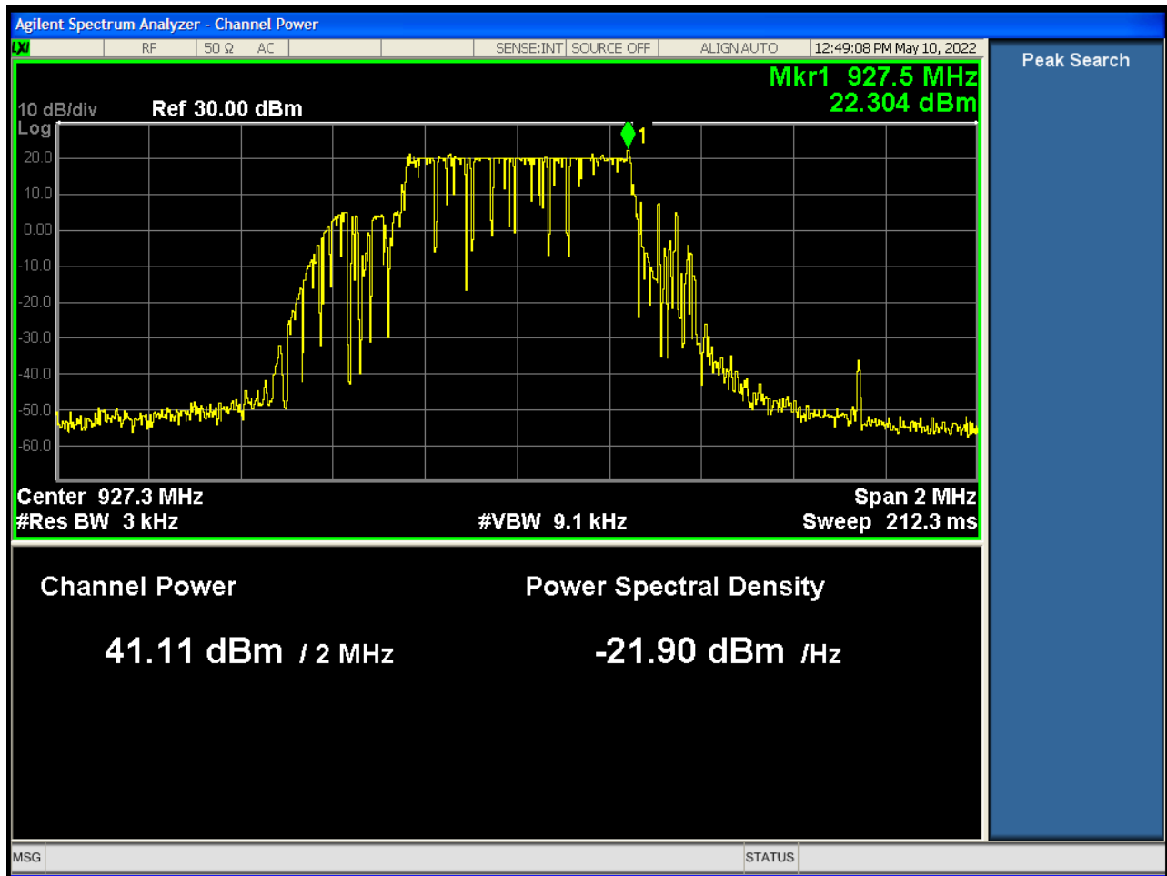
Power Spectral Density – High Channel
