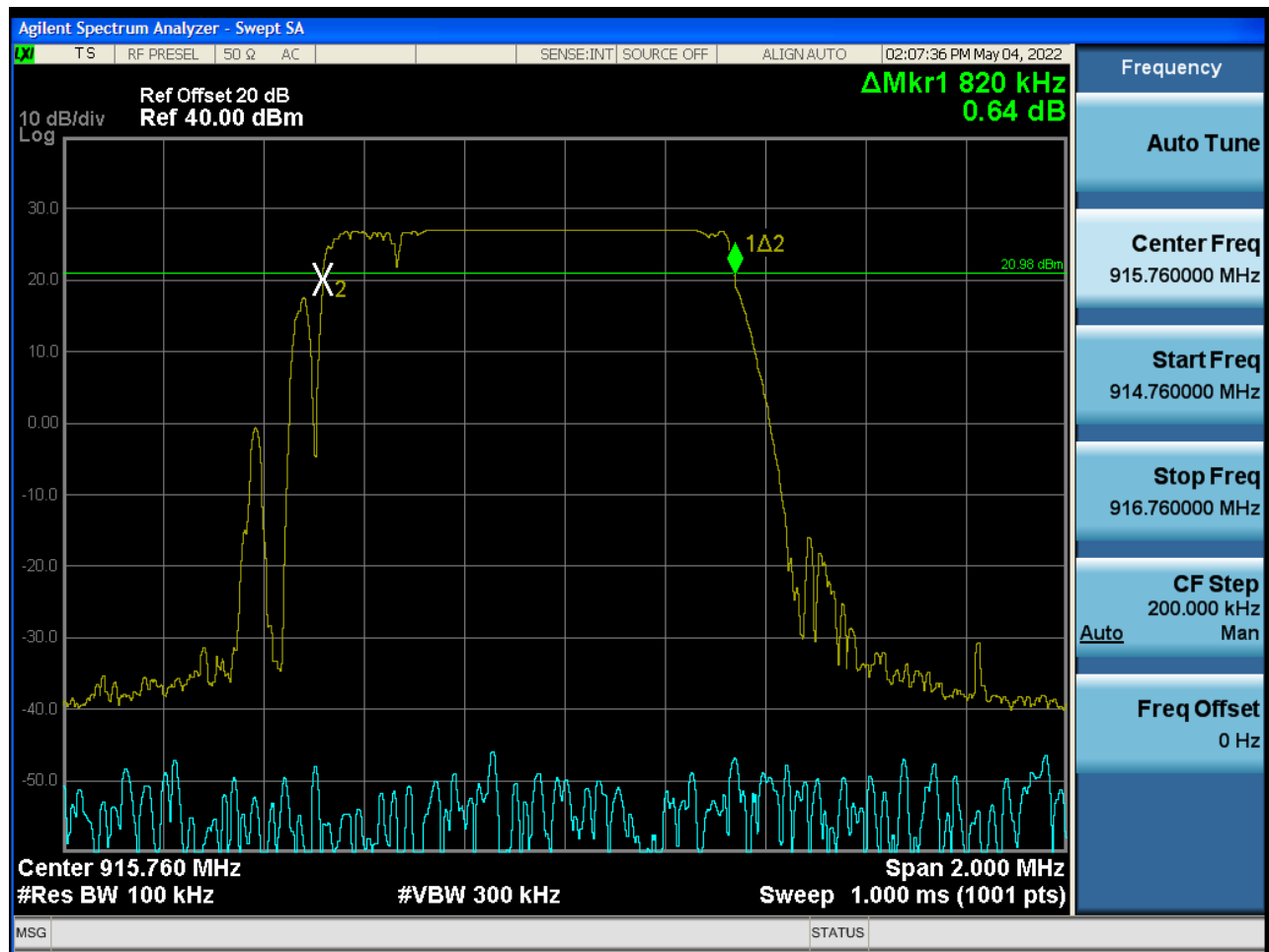
DTS Bandwidth – Middle Channel
