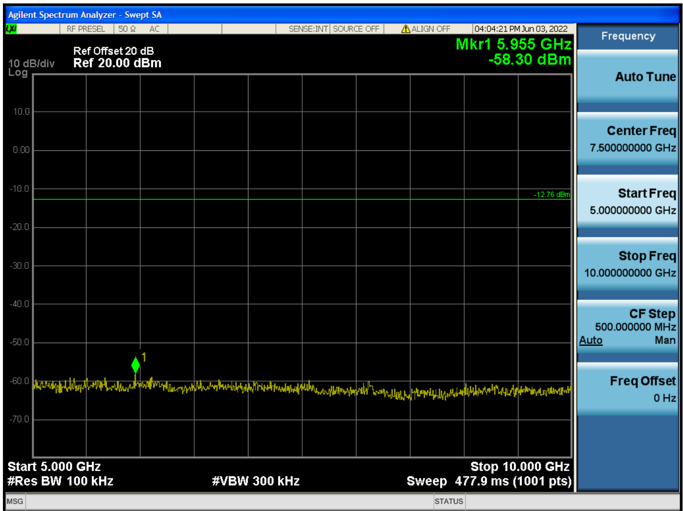
RF Antenna Conducted Test – Mid Channel – 5 GHz to 10 GHz
