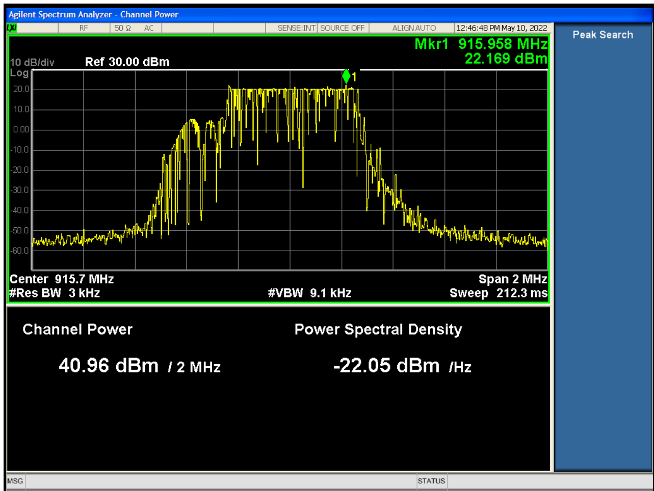
Power Spectral Density – Middle Channel
