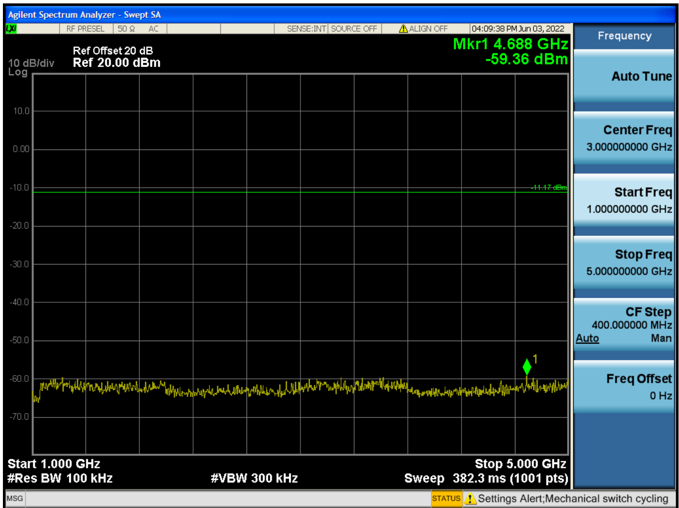
RF Antenna Conducted Test – Low Channel – 1 GHz to 5 GHz
