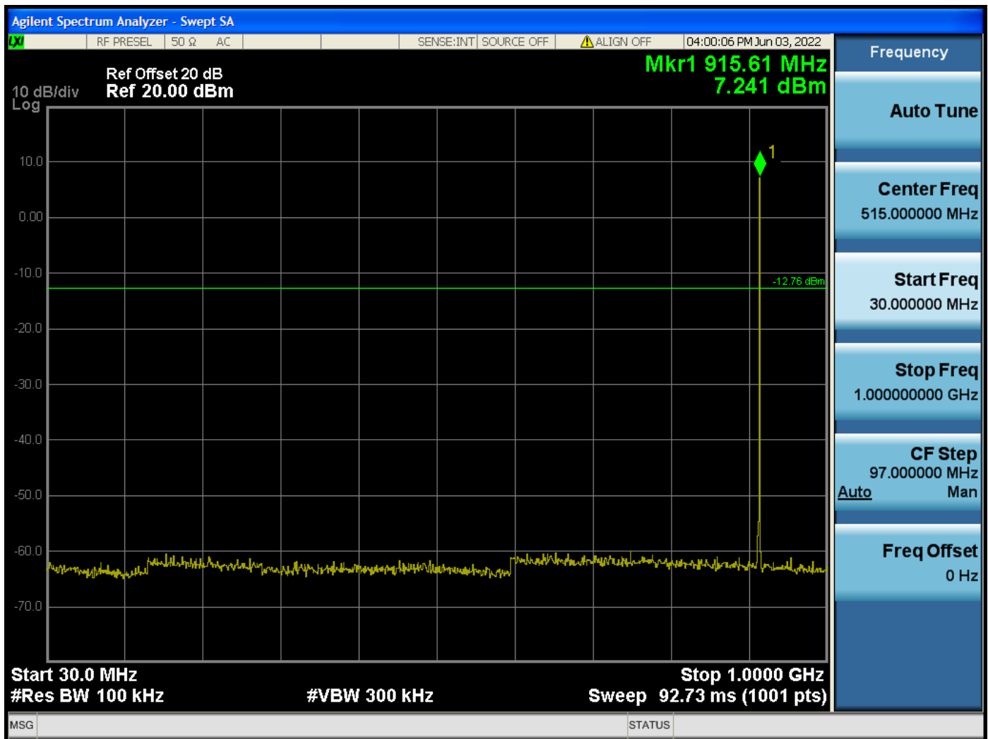
RF Antenna Conducted Test – Mid Channel – 30 MHz to 1 GHz
