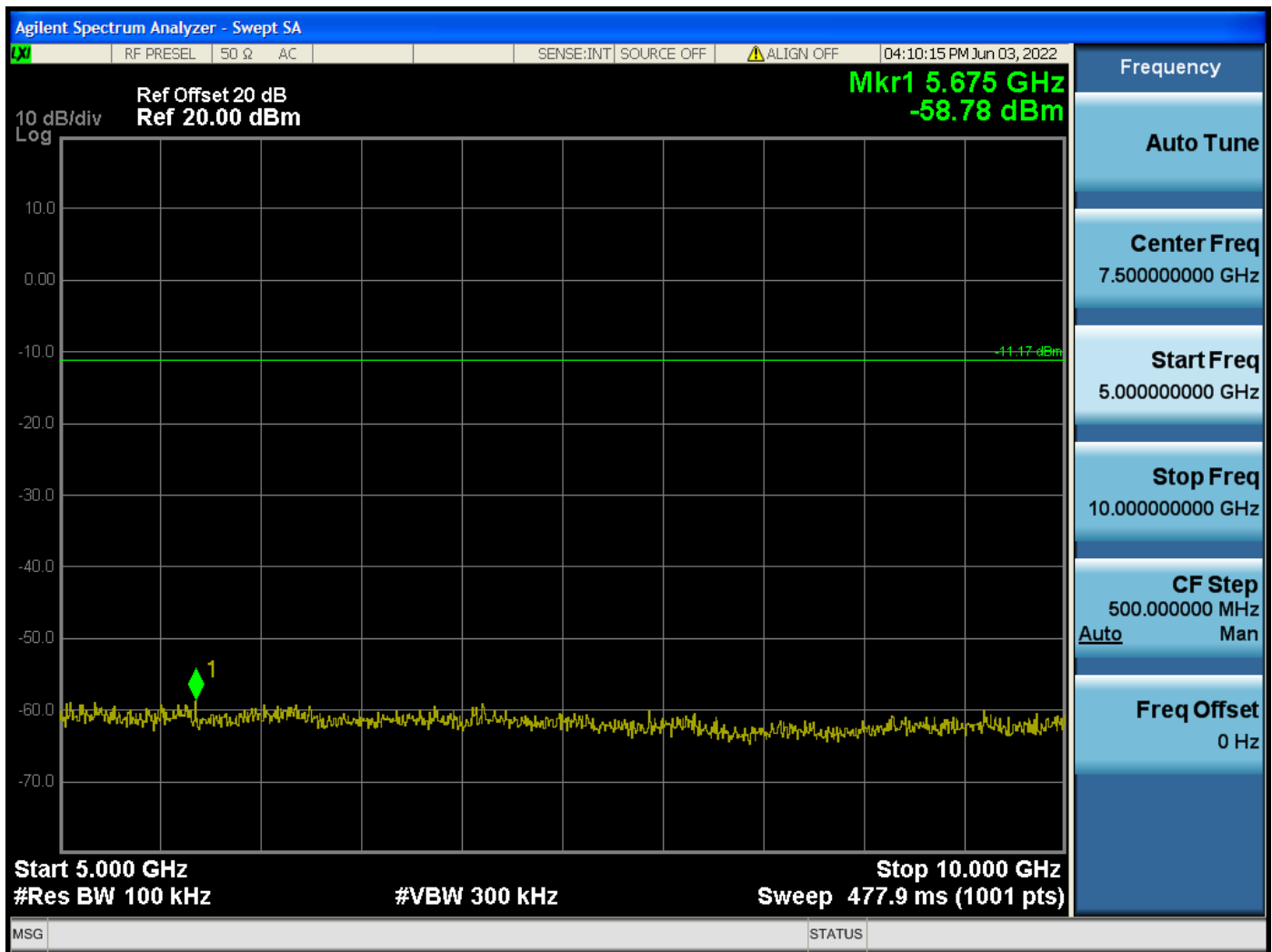
RF Antenna Conducted Test – Low Channel – 5 GHz to 10 GHz
