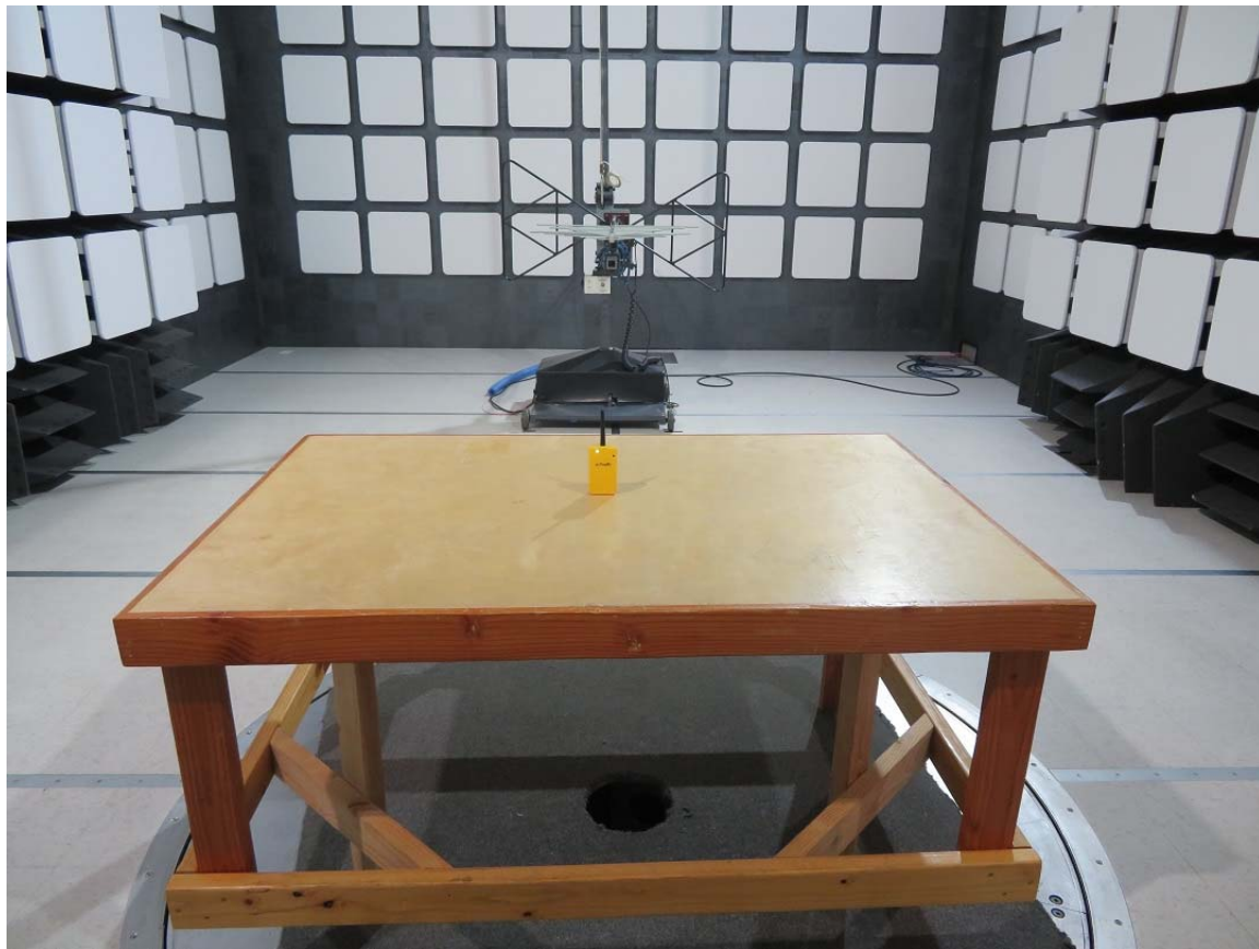
Radiated Emissions below 1 GHz
