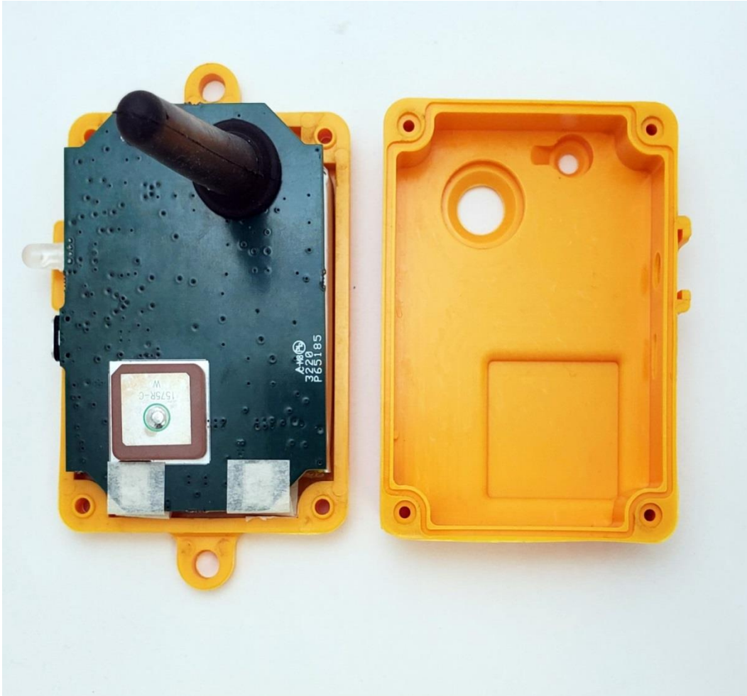
MMI-TRAKR2 – Internal View, Top
