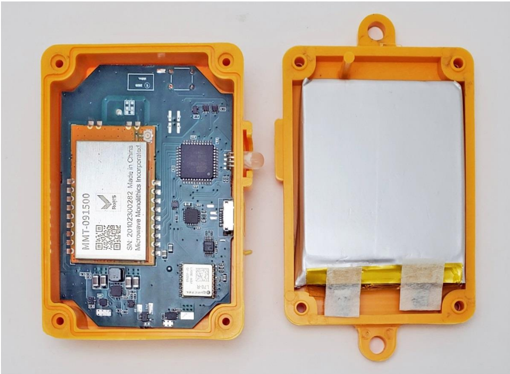
MMI-TRAKR2 – Internal View, Bottom
