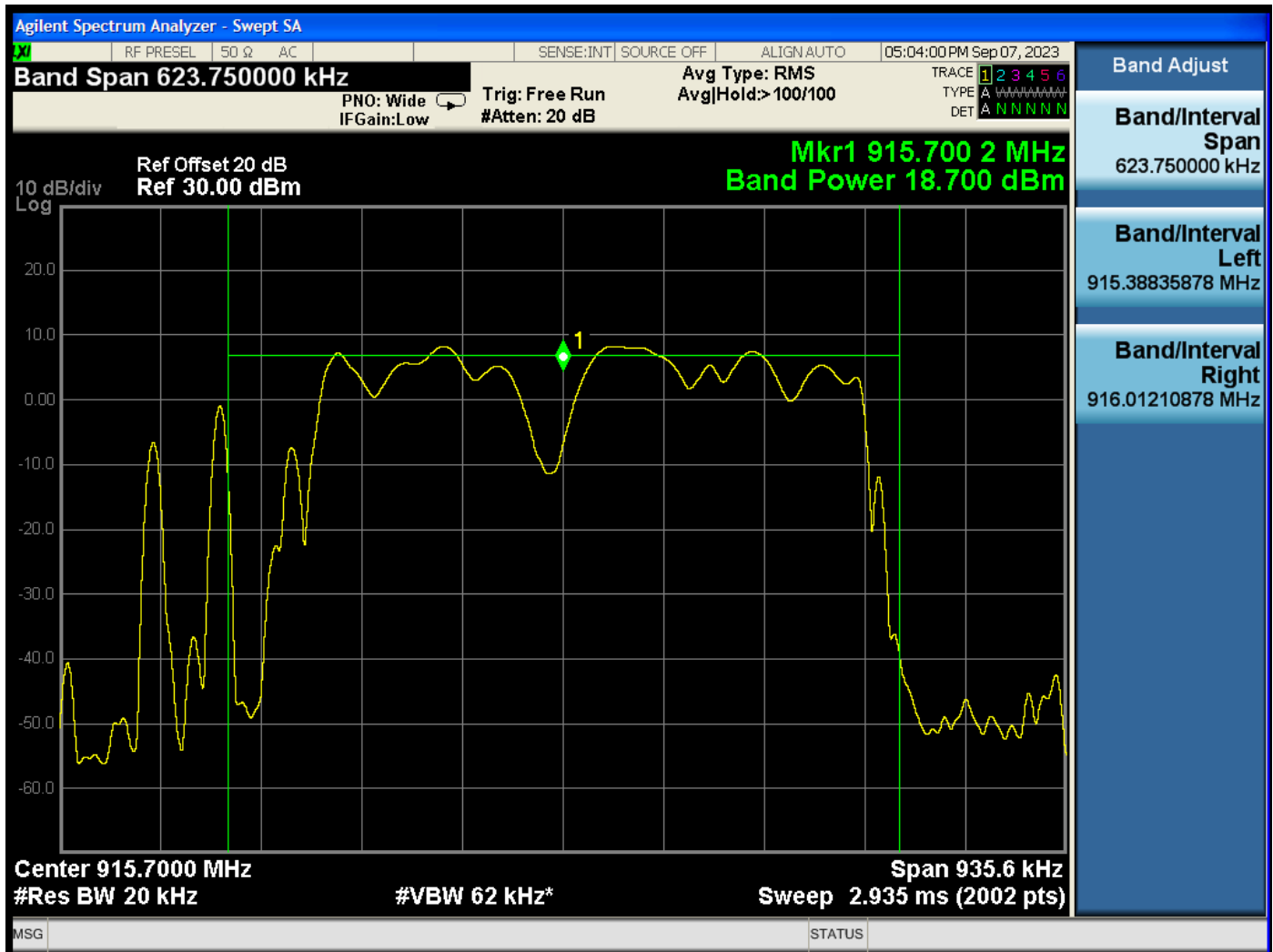
Maximum Conducted Output Power - Middle Channel
