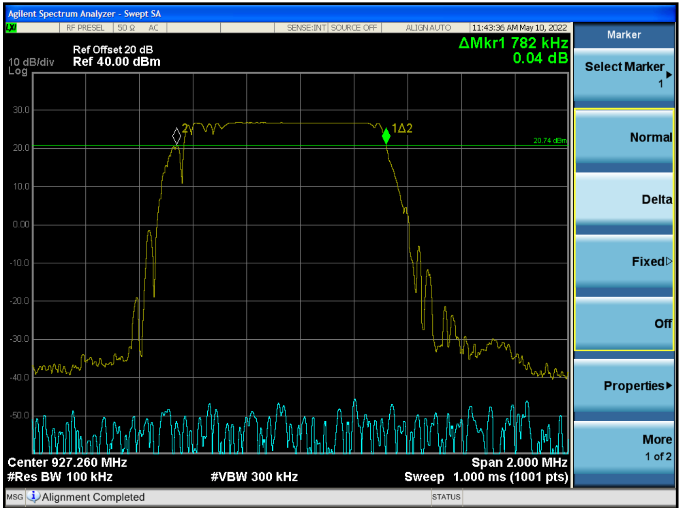
DTS Bandwidth – High Channel
