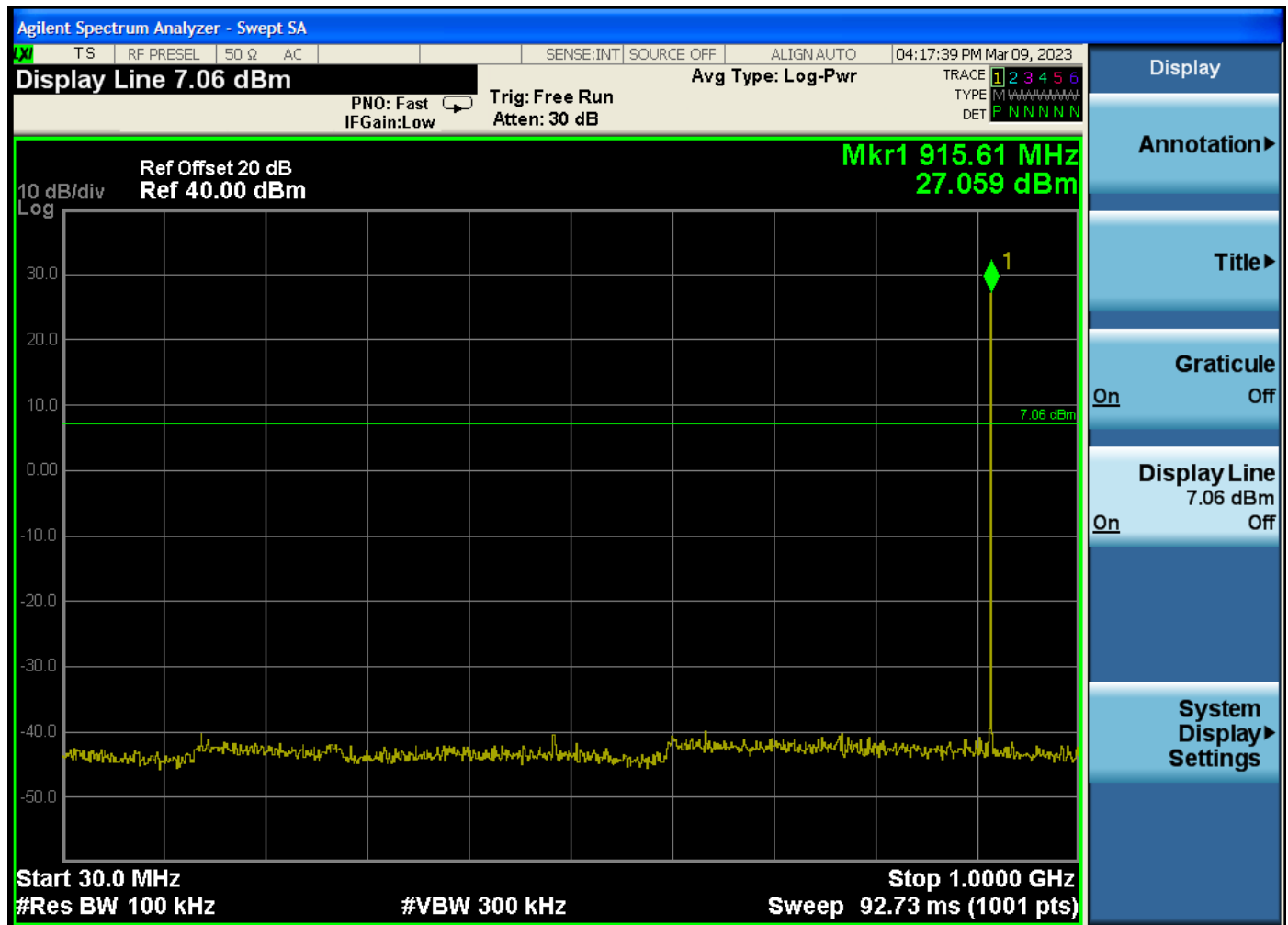
RF Antenna Conducted Test – Middle Channel – 30 MHz to 1 GHz
