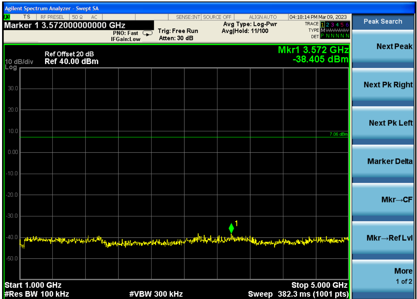
RF Antenna Conducted Test – Middle Channel – 1 GHz to 5 GHz
