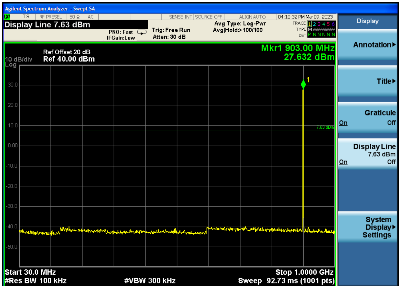
RF Antenna Conducted Test – Low Channel – 30 MHz to 1 GHz
