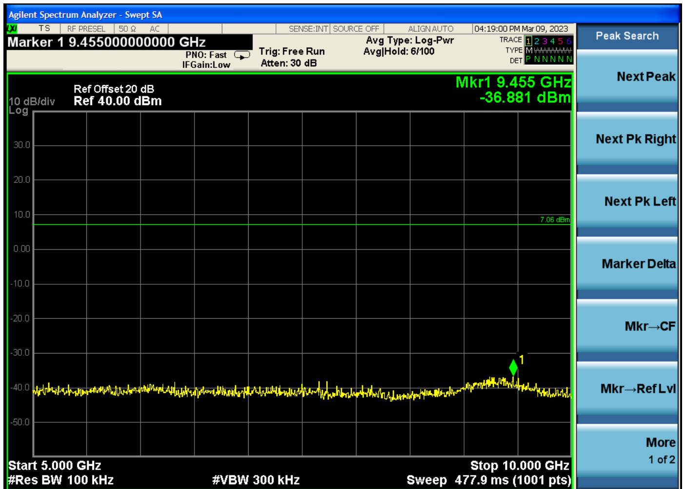
RF Antenna Conducted Test – Middle Channel – 5 GHz to 10 GHz
