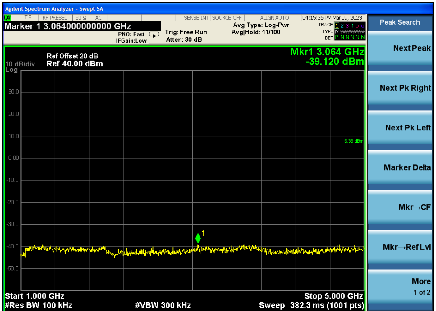
RF Antenna Conducted Test – High Channel – 1 GHz to 5 GHz
