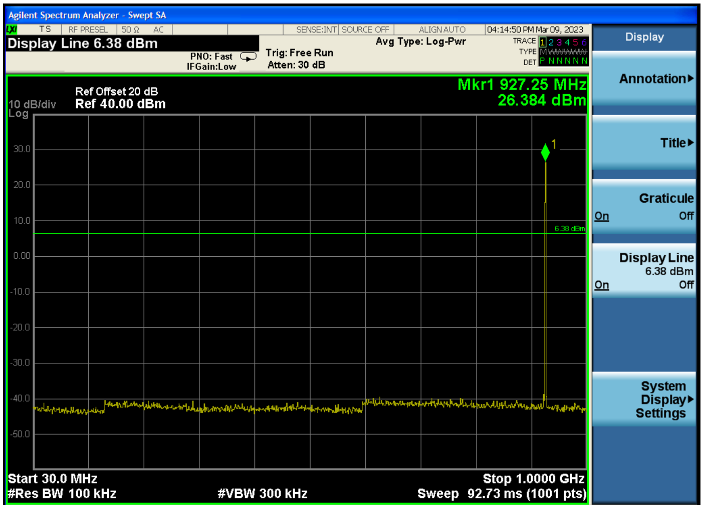
RF Antenna Conducted Test – High Channel – 30 MHz to 1 GHz
