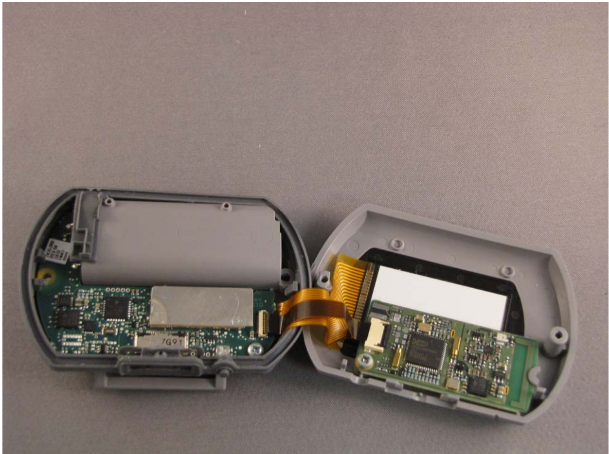
Figure 1 Model 3150 Open Main PWBA on left SABER over LCD on right
