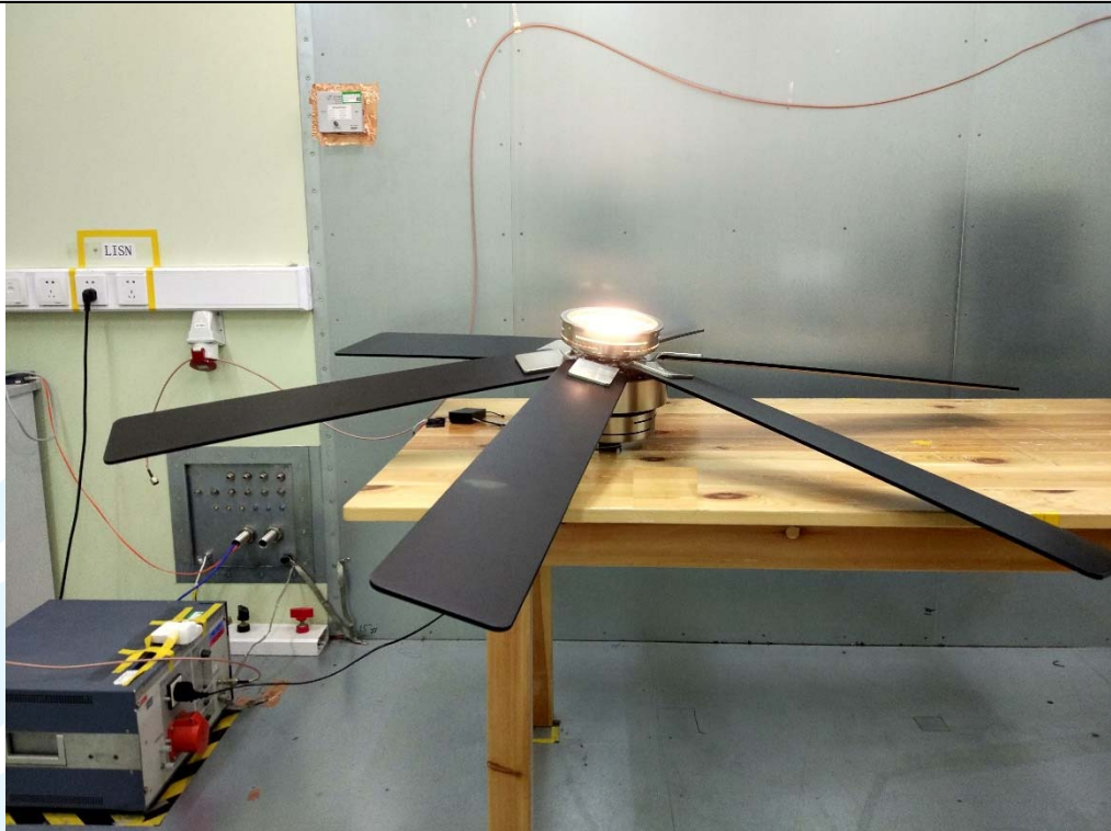
Conducted Emission Test Setup-3 - Mode 1
