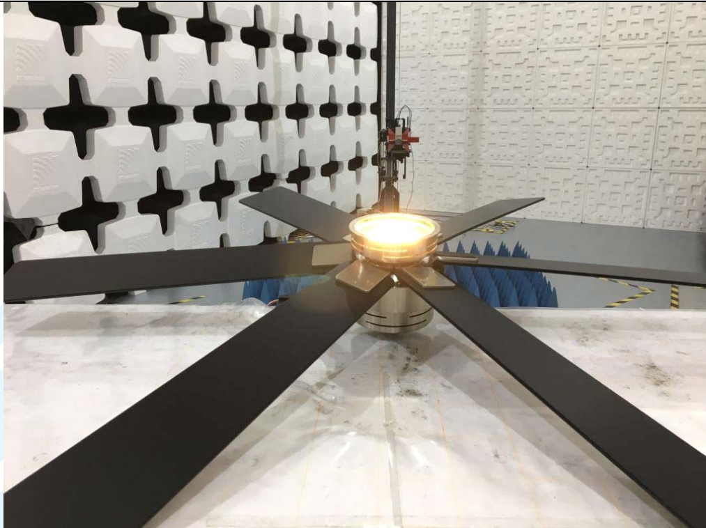
Radiated emission Test Setup-2 (Above 1 GHz) - Mode 1
