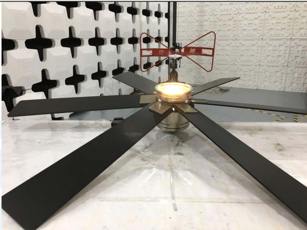
Radiated emission Test Setup-1 (30 MHz~1 GHz) - Mode 1
