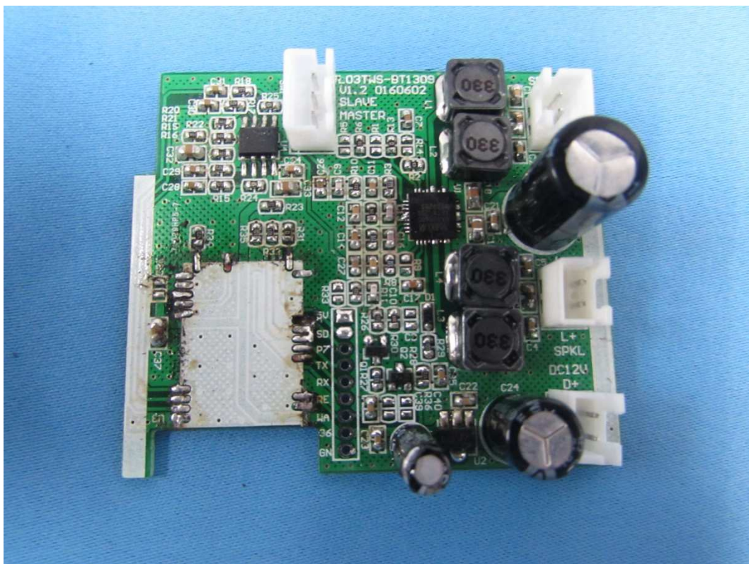
Control PCB view (remove Bluetooth)
