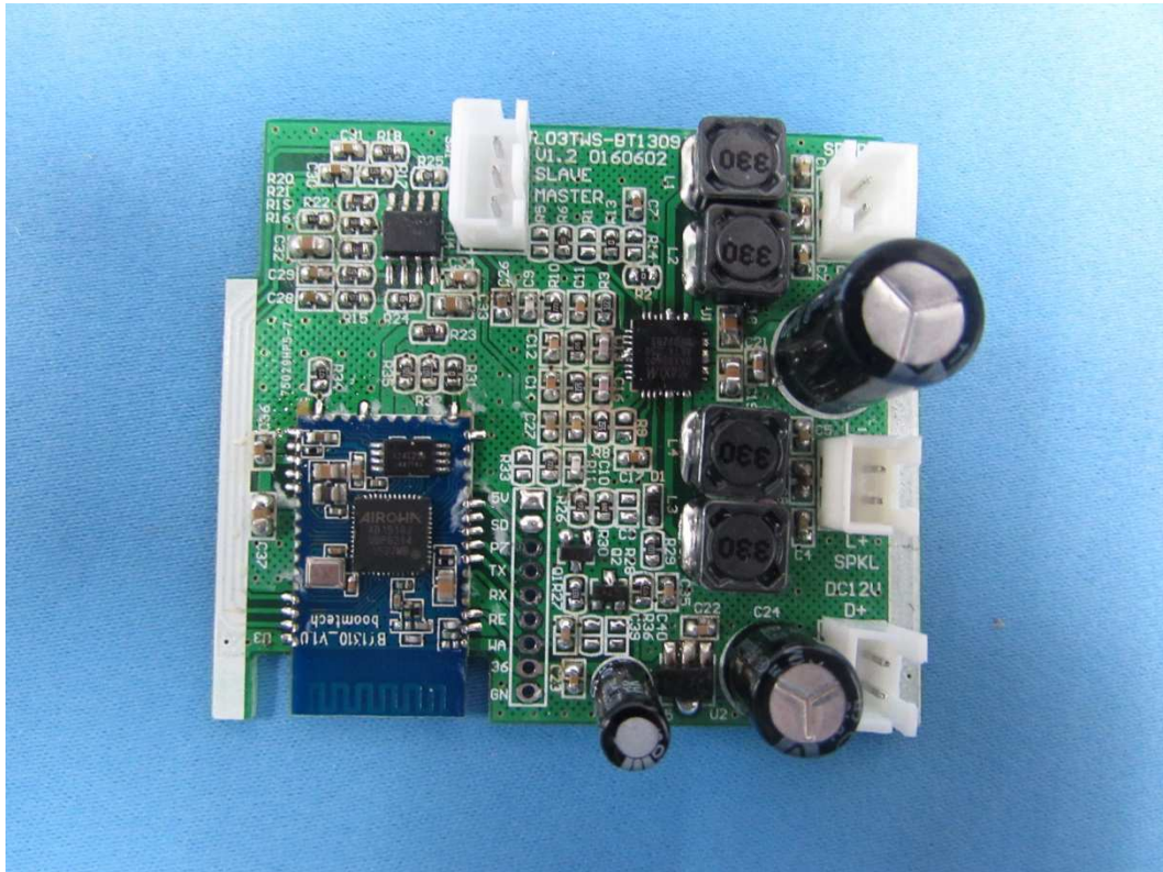
Control PCB view
