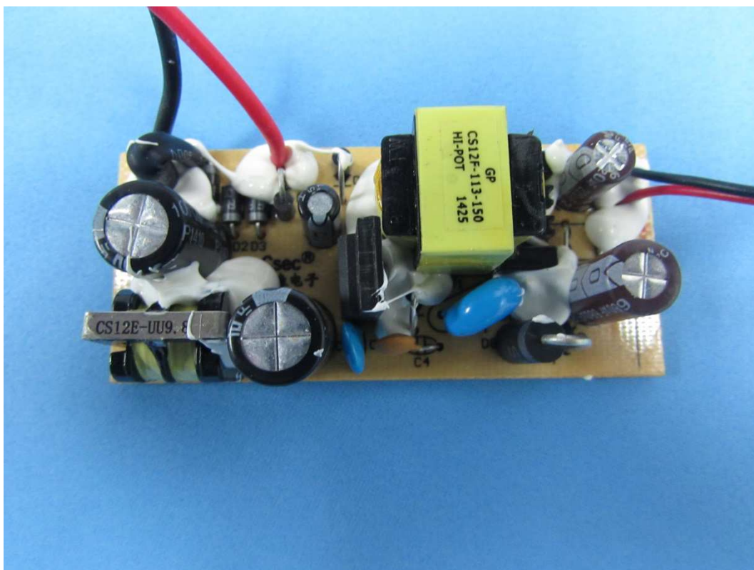
Power PCB view
