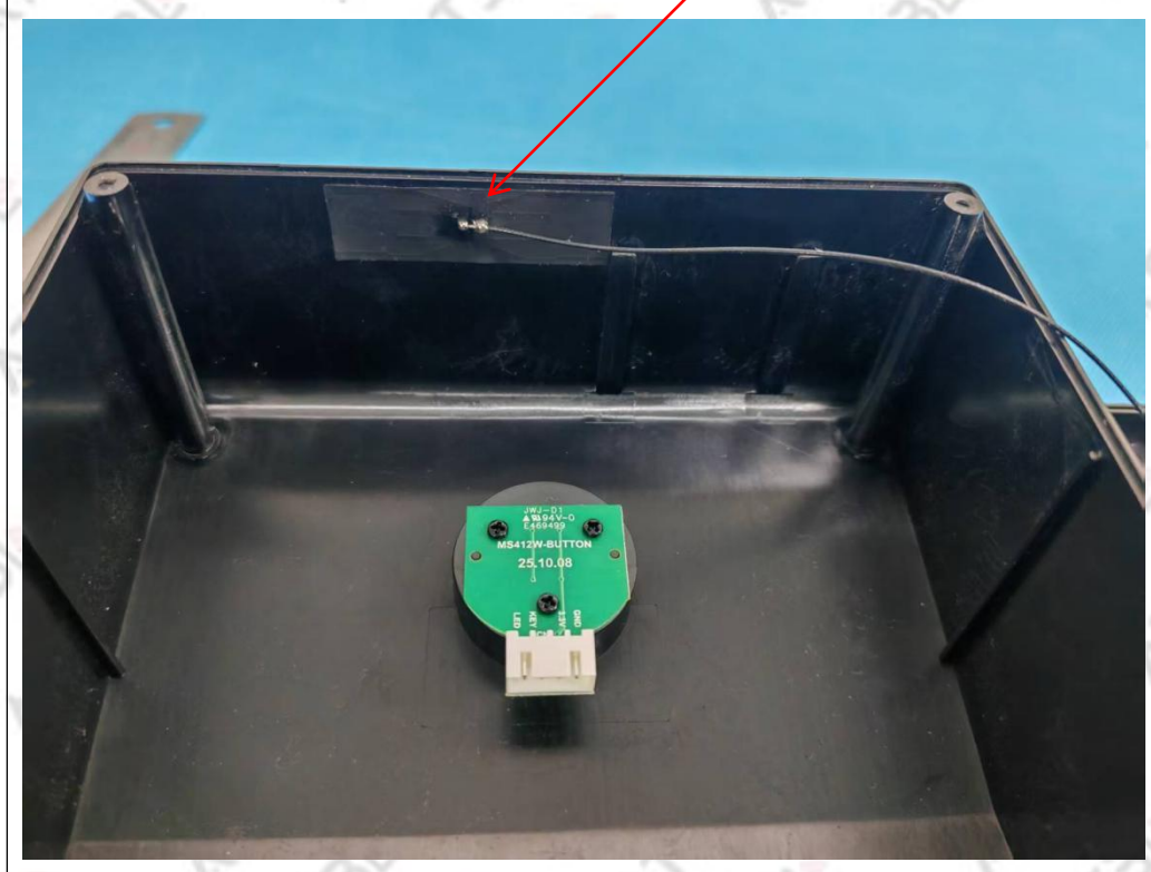
BT&2.4G WiFi_ANT
