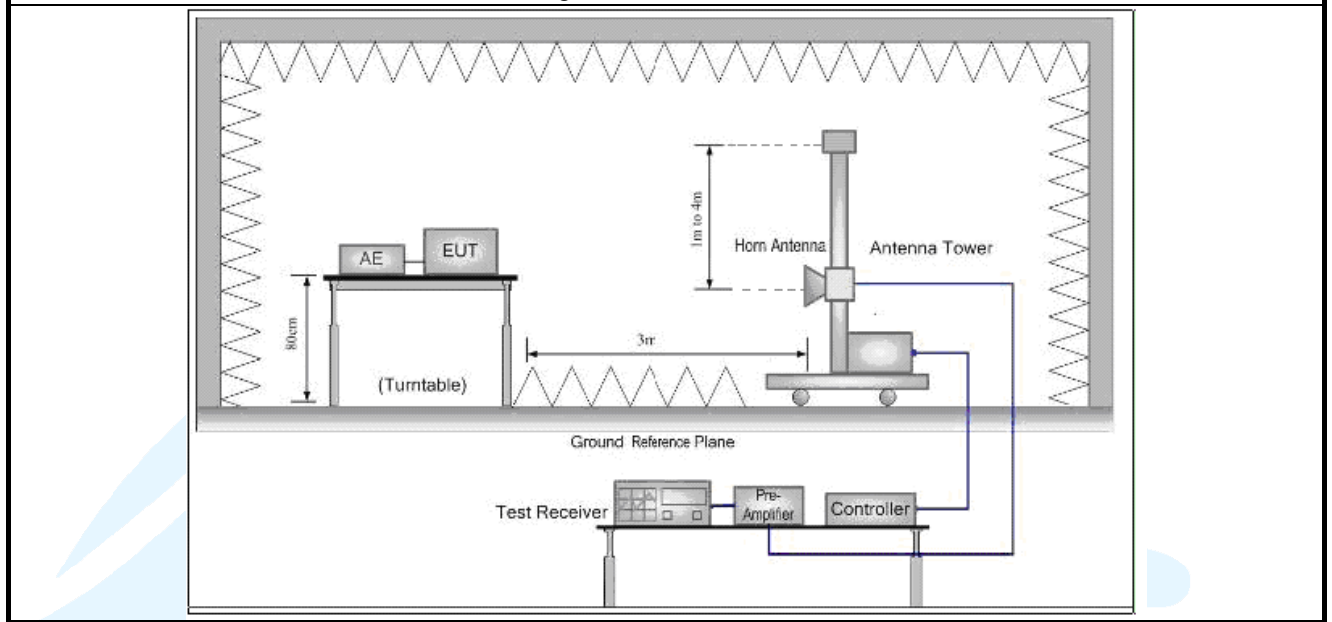
Figure 2. Above 1GHz
