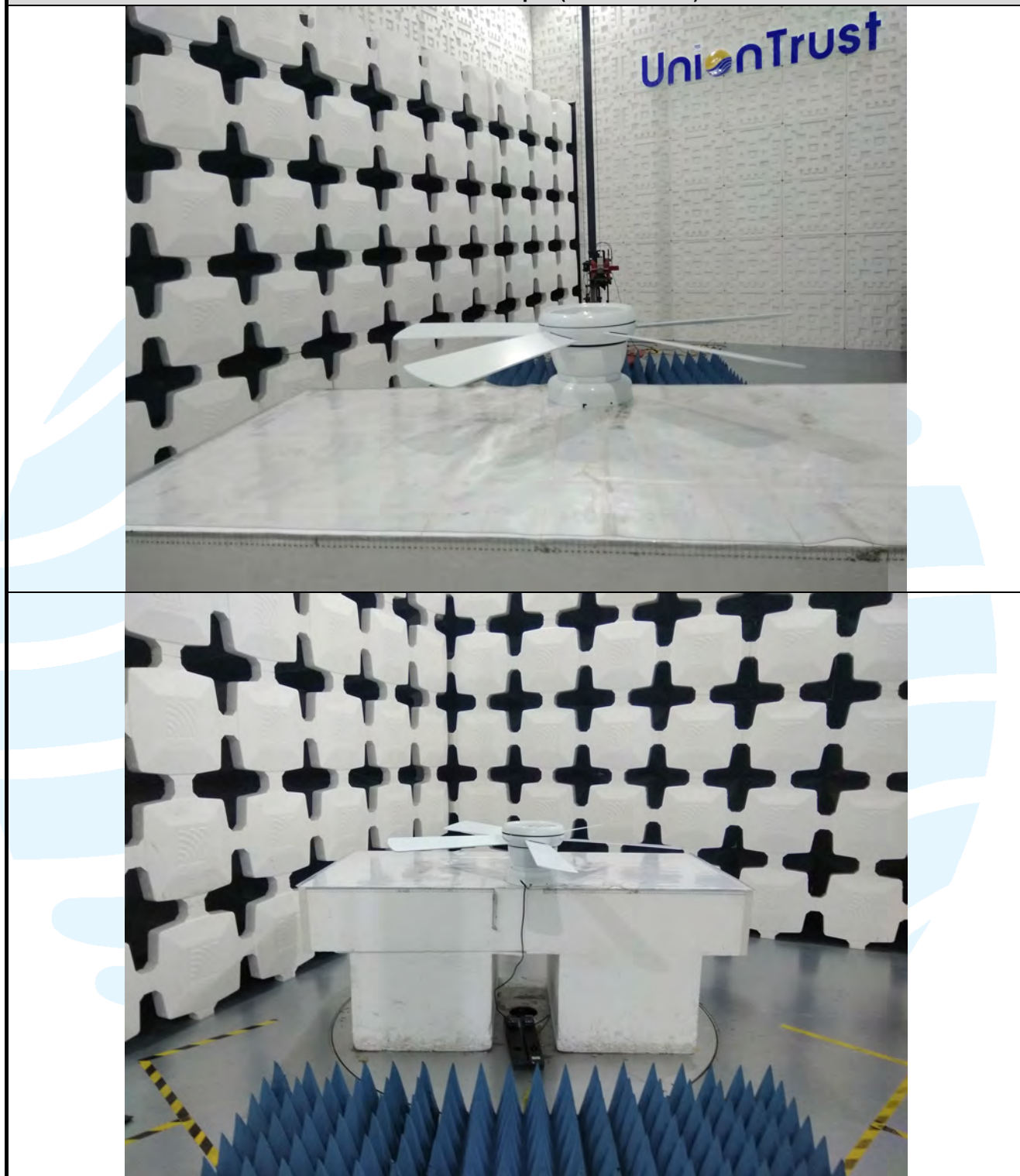
Radiated emission Test Setup-2 (Above 1 GHz) - Mode 1
