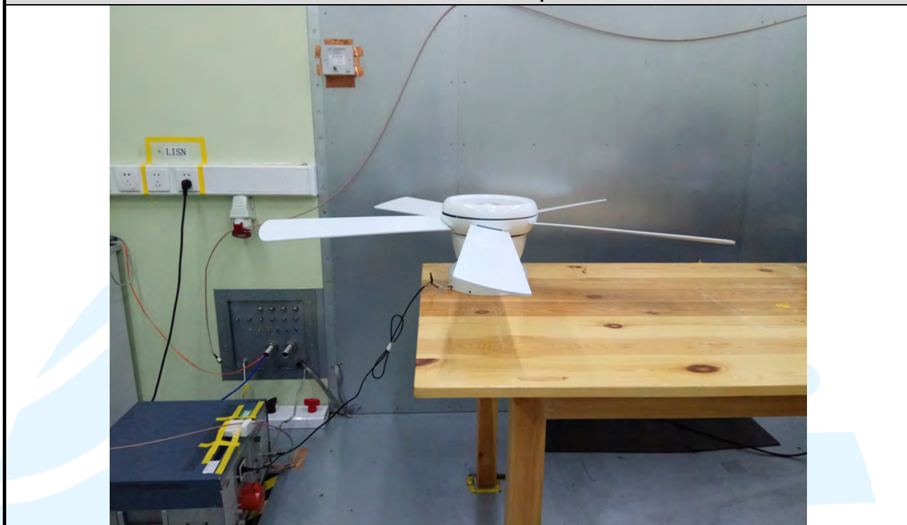
Conducted Emission Test Setup-3 - Mode 1
