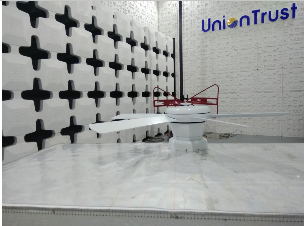
Radiated emission Test Setup-1 (30 MHz~1 GHz) - Mode 1
