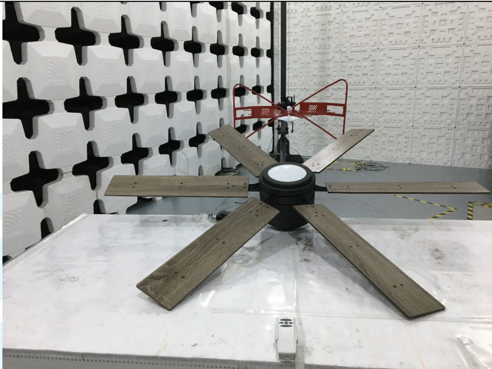
Radiated emission Test Setup-1 (30 MHz~1 GHz)
