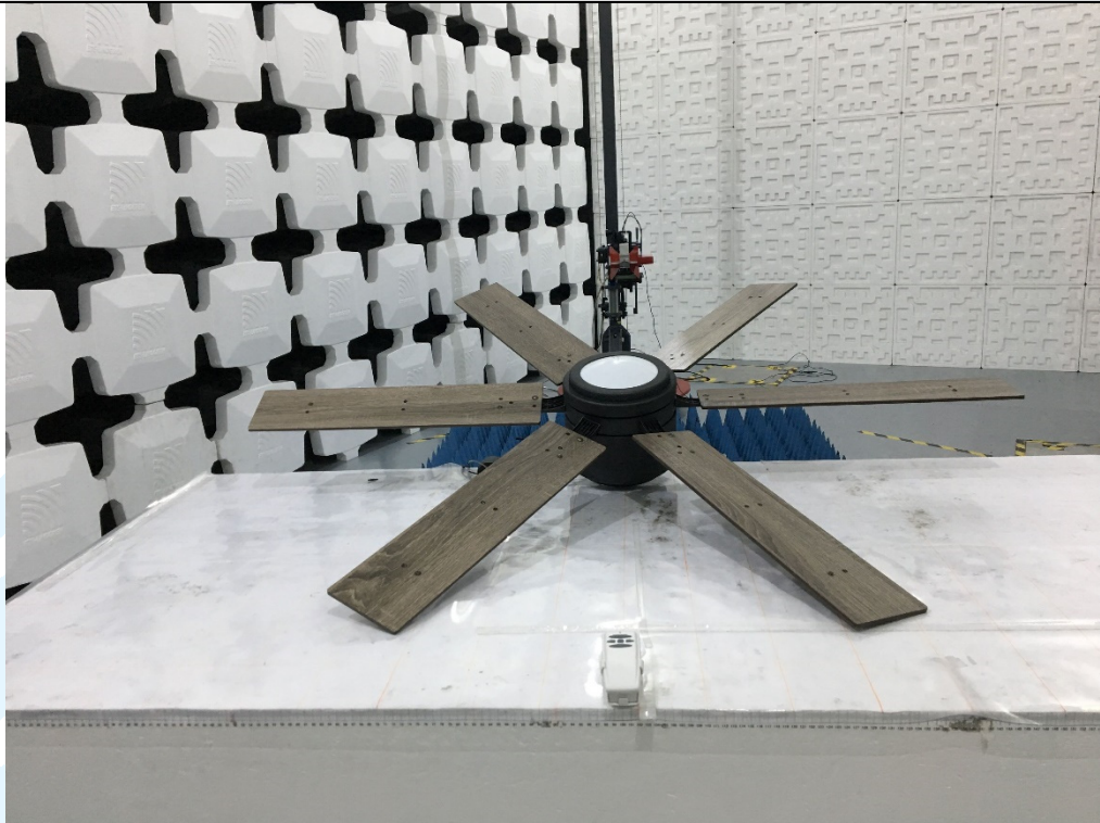
Radiated emission Test Setup-2 (Above 1 GHz)
