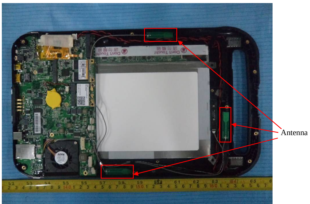
EUT – Cover off View (8pin, without Halo LED)
