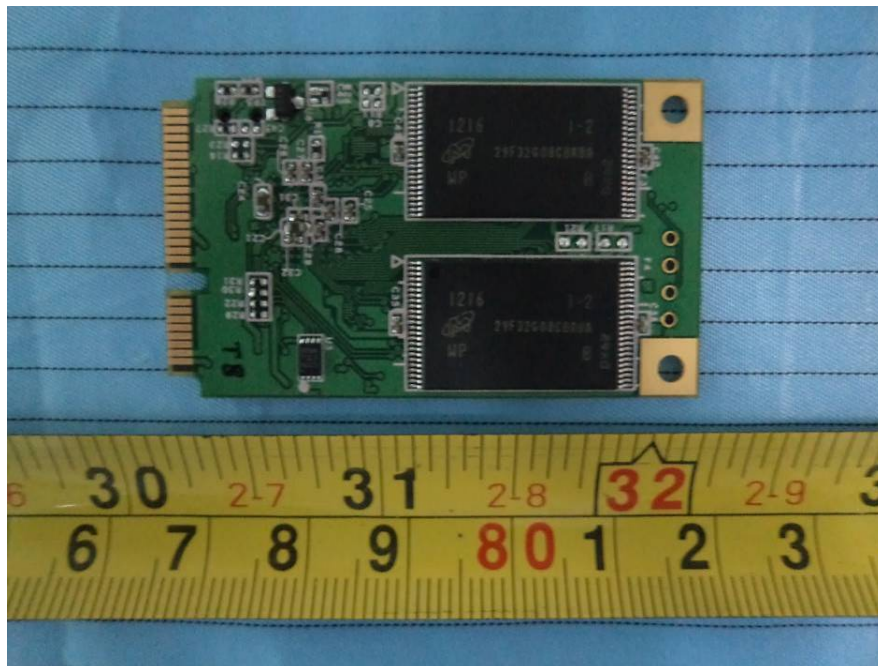
EUT – 16G Disk Board Bottom View
