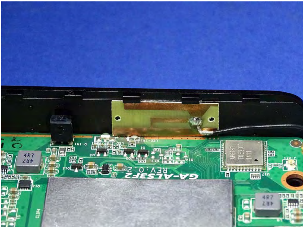
(7) EUT Photo-Antenna
