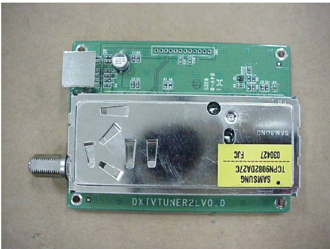
<Tuner board front>
