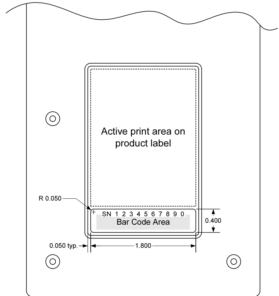
Base Unit Serial # label 500-00009-00 dimensions and placement on product label
