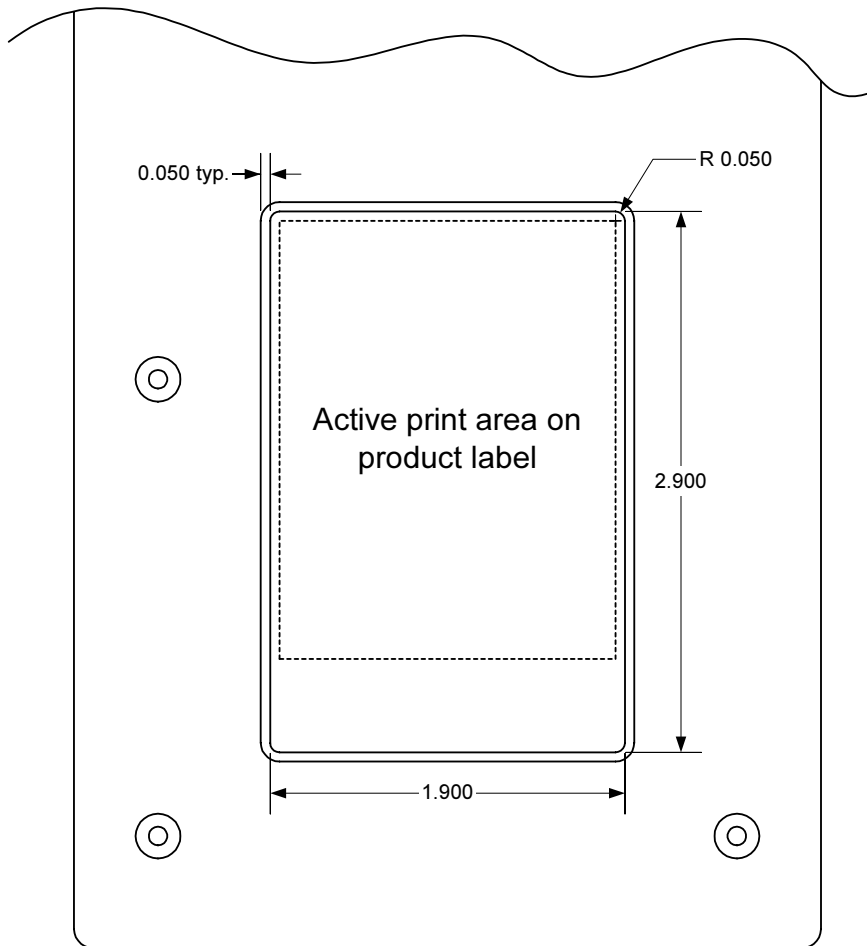
Product label 500-00006-00 dimensions and placement on Base Unit
