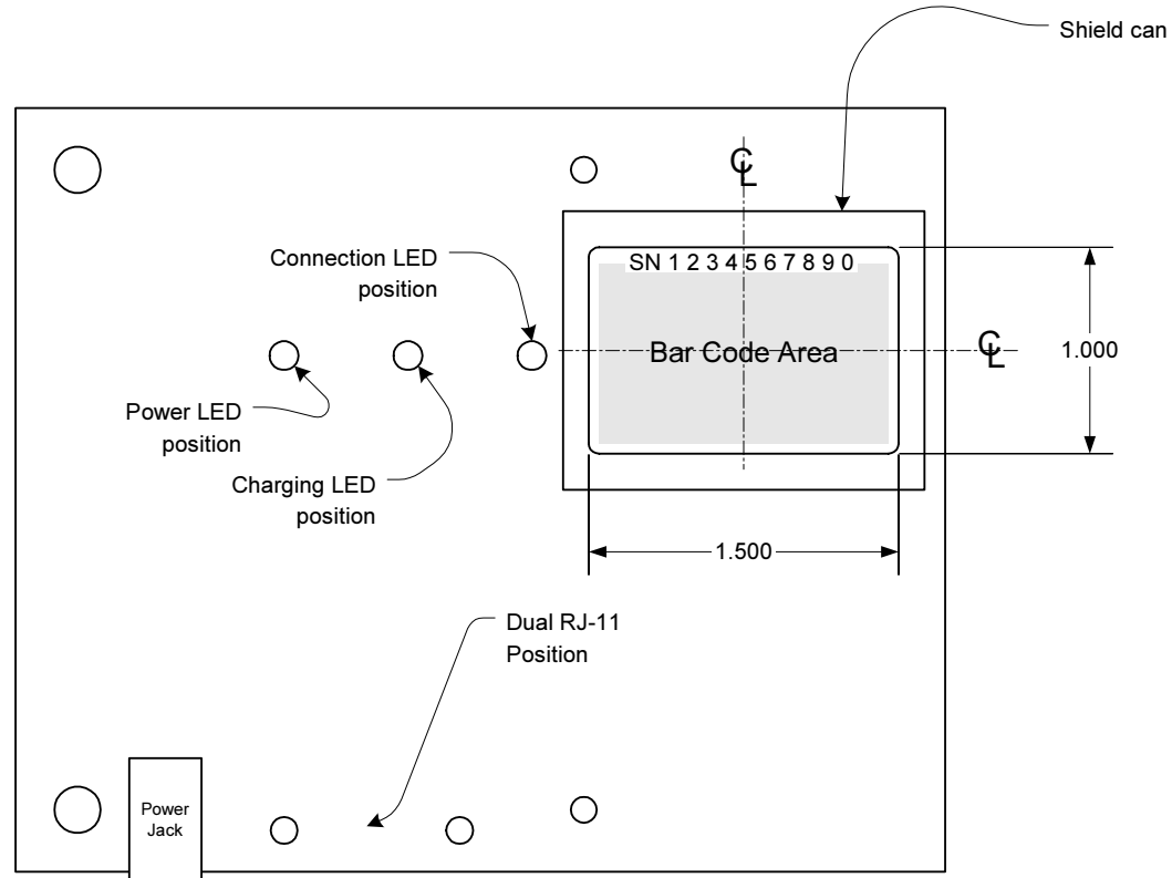
Component Side (Front) View
