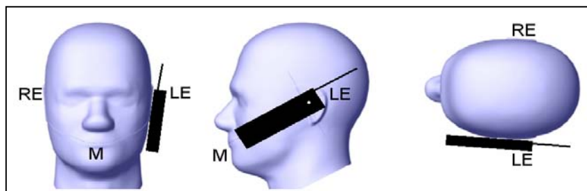
Figure 6 Front, Side and Top View of Cheek/Touch Position
