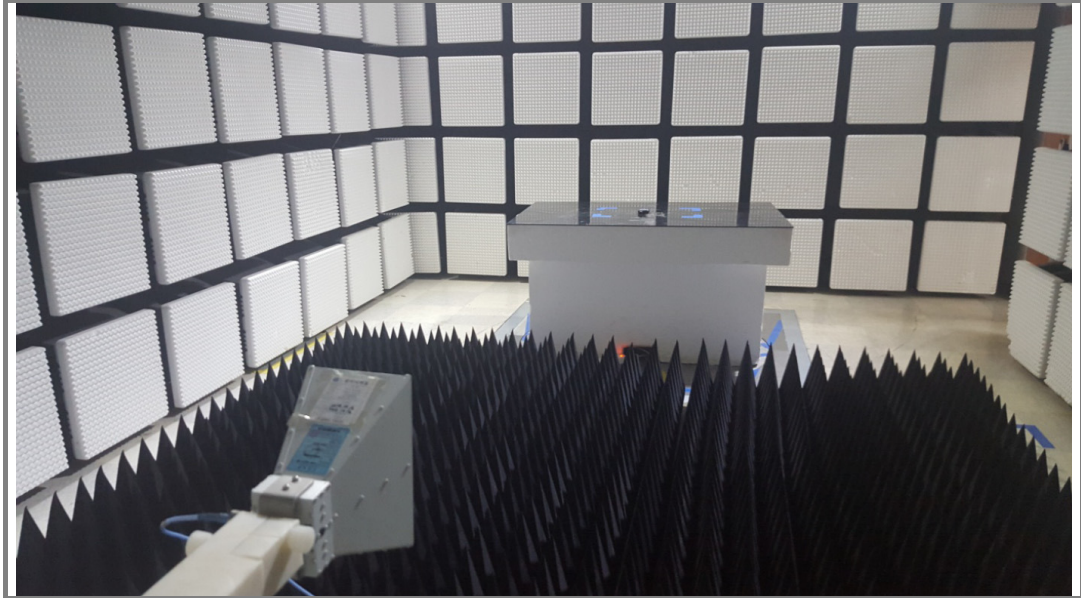
Photo of radiated spurious emission at above 1 000 MHz
