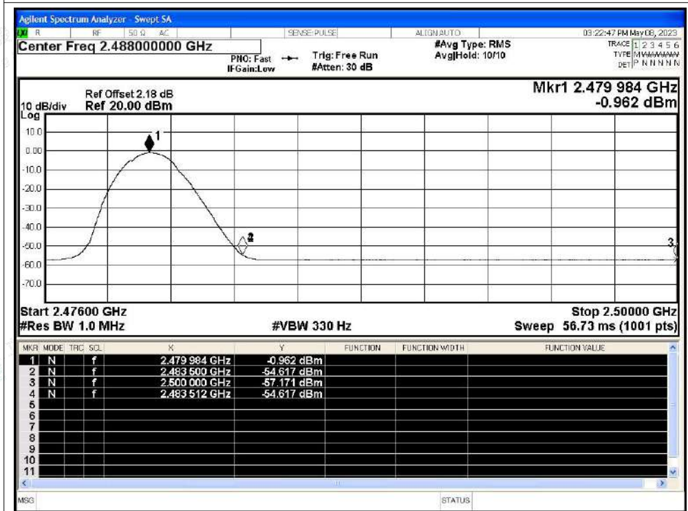
Restrict Band NVNT 2-DH5 2480MHz Ant1 No-Hopping Average
