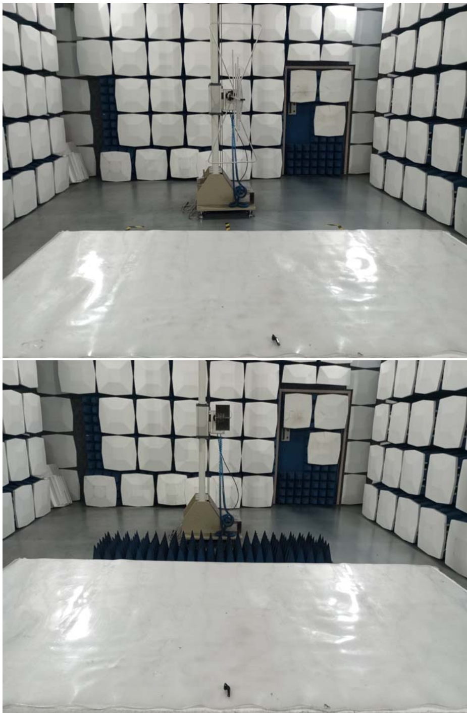
Radiated emission test view
