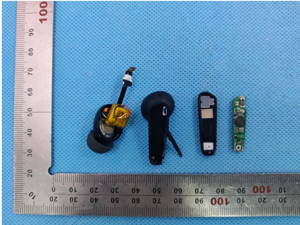
Open view of EUT(Left earphone)
