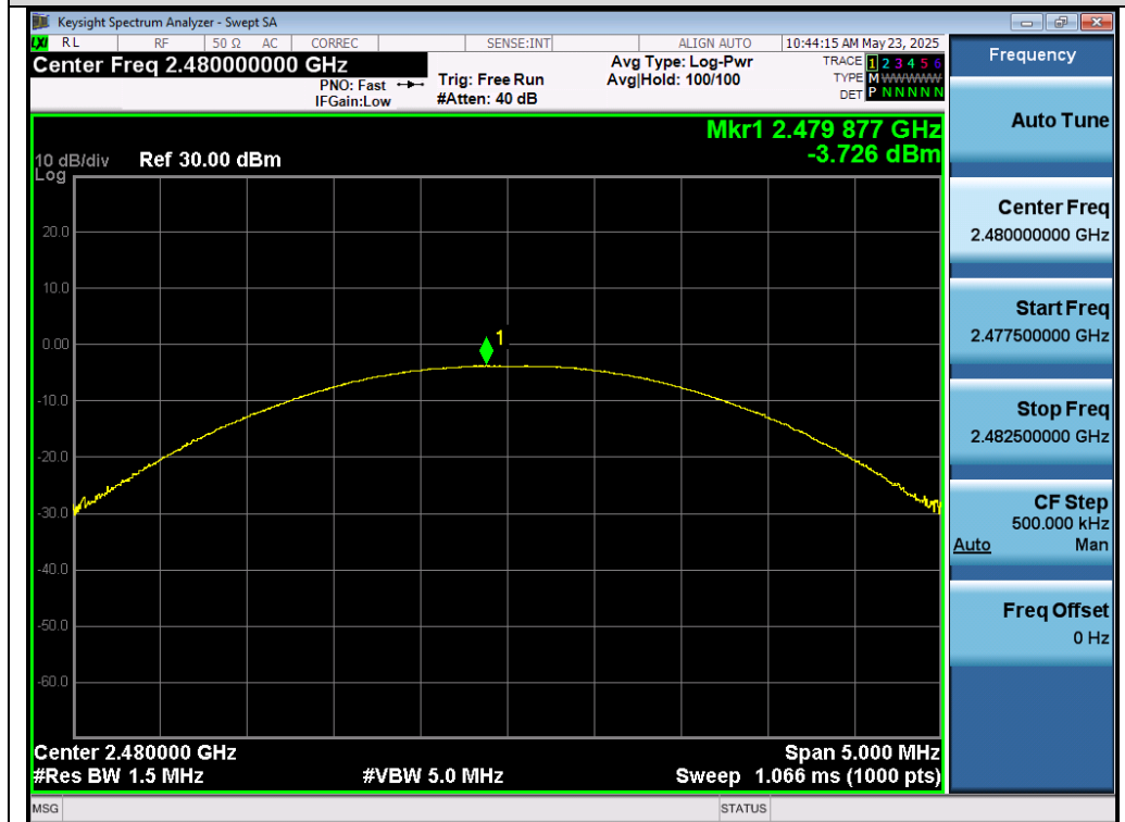
Test_Graph_EDR_ANT1_2480_2Mbps_Peak Power
