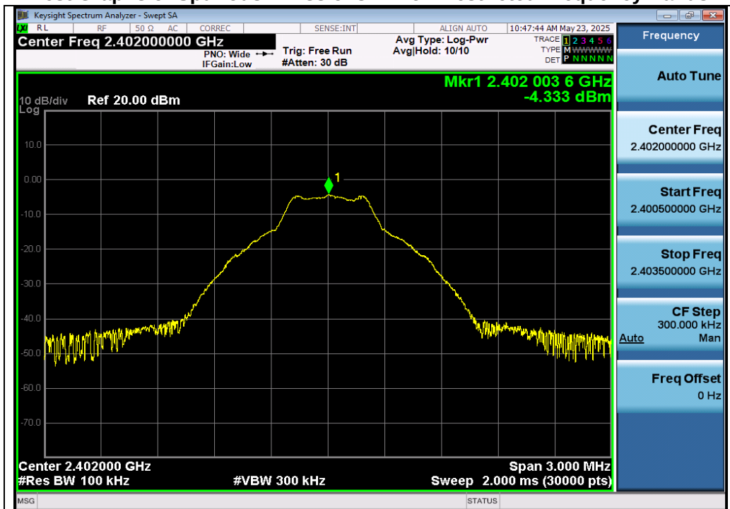
Test_Graph_BR_ANT1_2402_1Mbps_Reference Level
