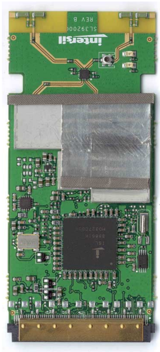
ISL39200C PCB front with shield
