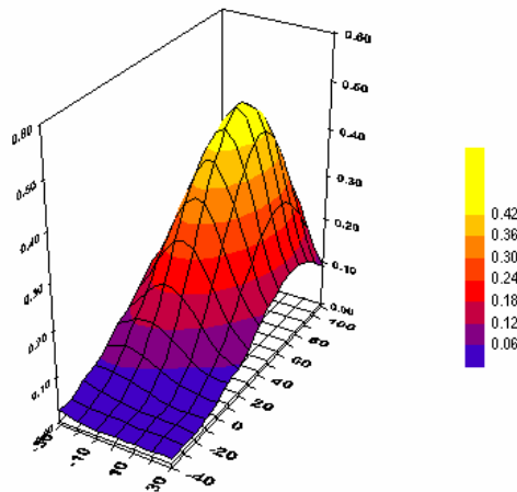
Figure 5.6.5.3. Area scan
