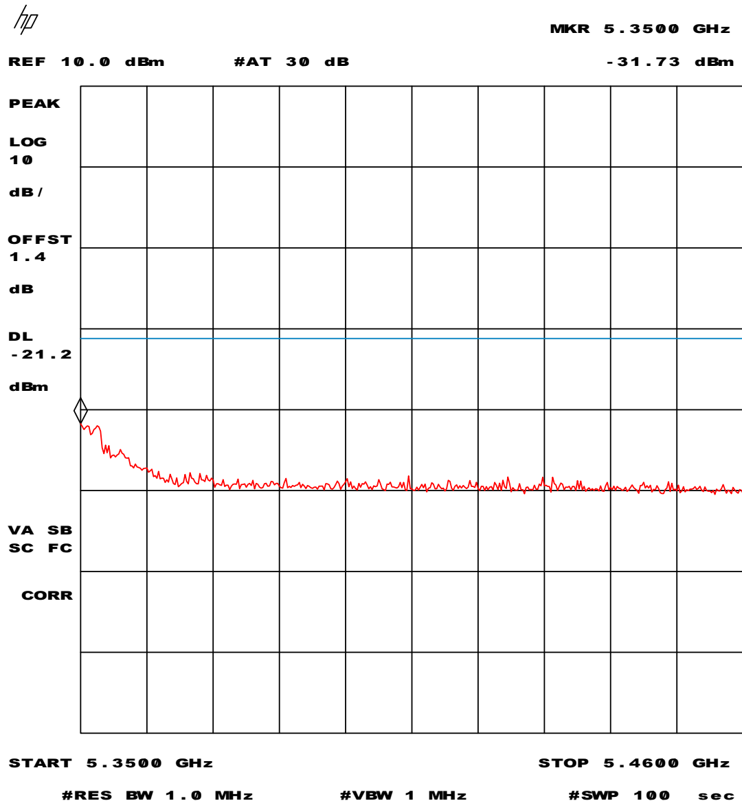
Plot 42 - Peak measurement values in the 5.35 – 5.46 GHz restricted band of operation
