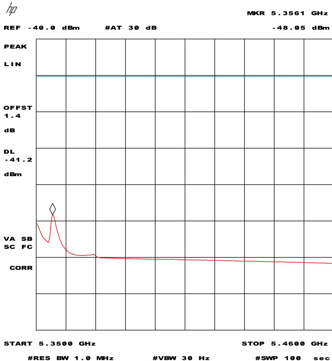
Plot 41 - Average measurement values in the 5.35 – 5.46 GHz restricted band of operation
