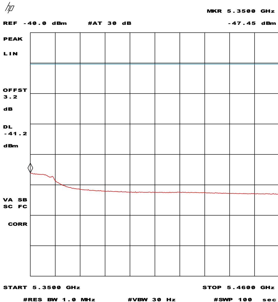
Plot 43 - Average measurement values in the 5.35 – 5.46 GHz restricted band of operation at -20 °C
