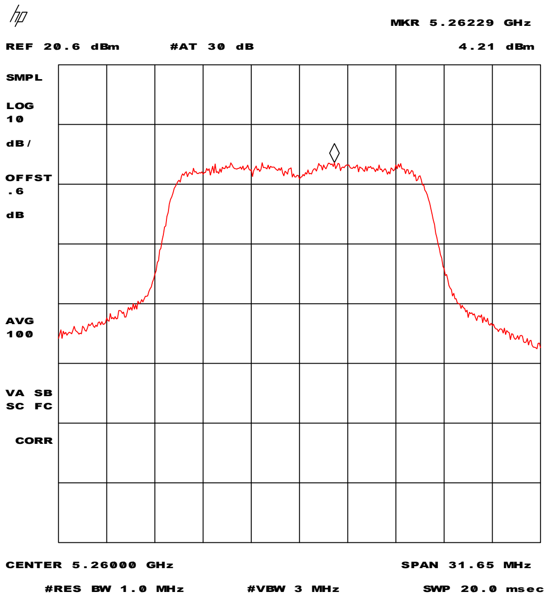
Plot 21 - Peak power spectral density (conducted) in any 1 MHz band.
