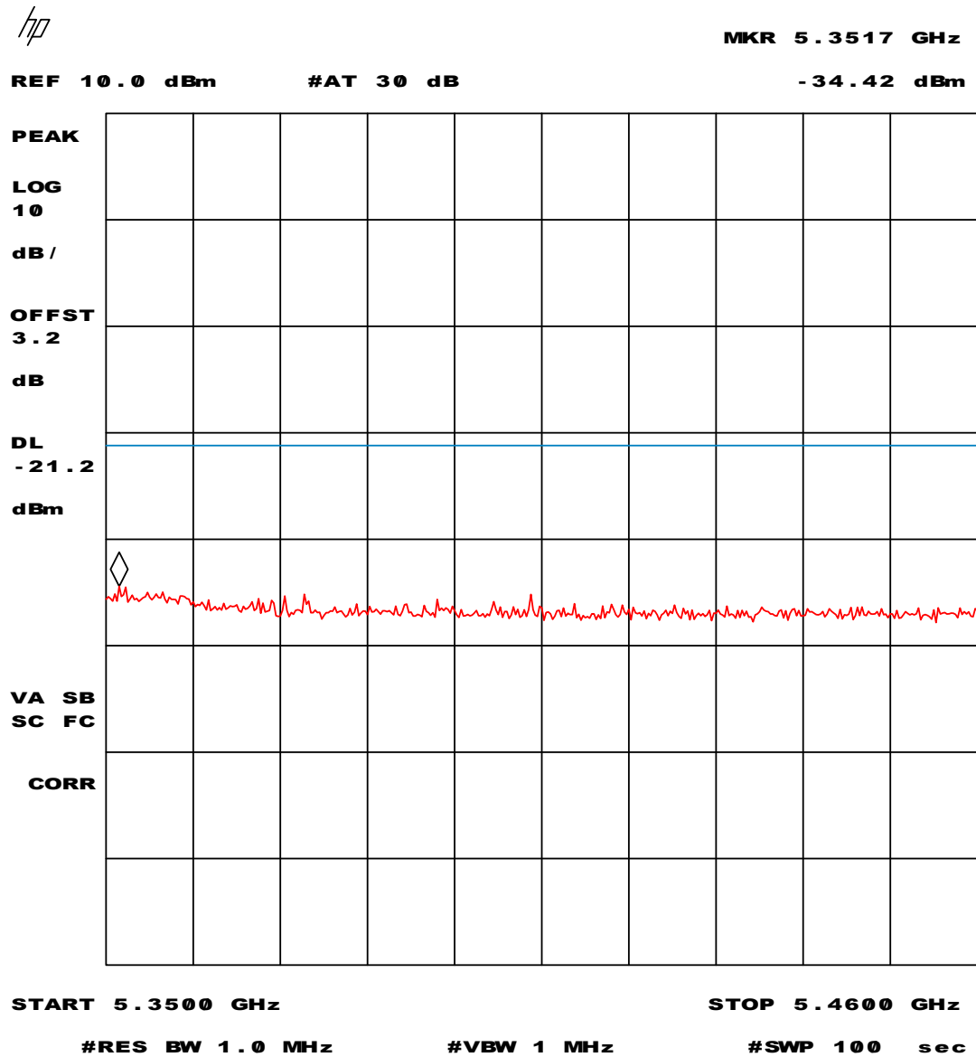
Plot 44 - Peak measurement values in the 5.35 – 5.46 GHz restricted band of operation at -20 °C
