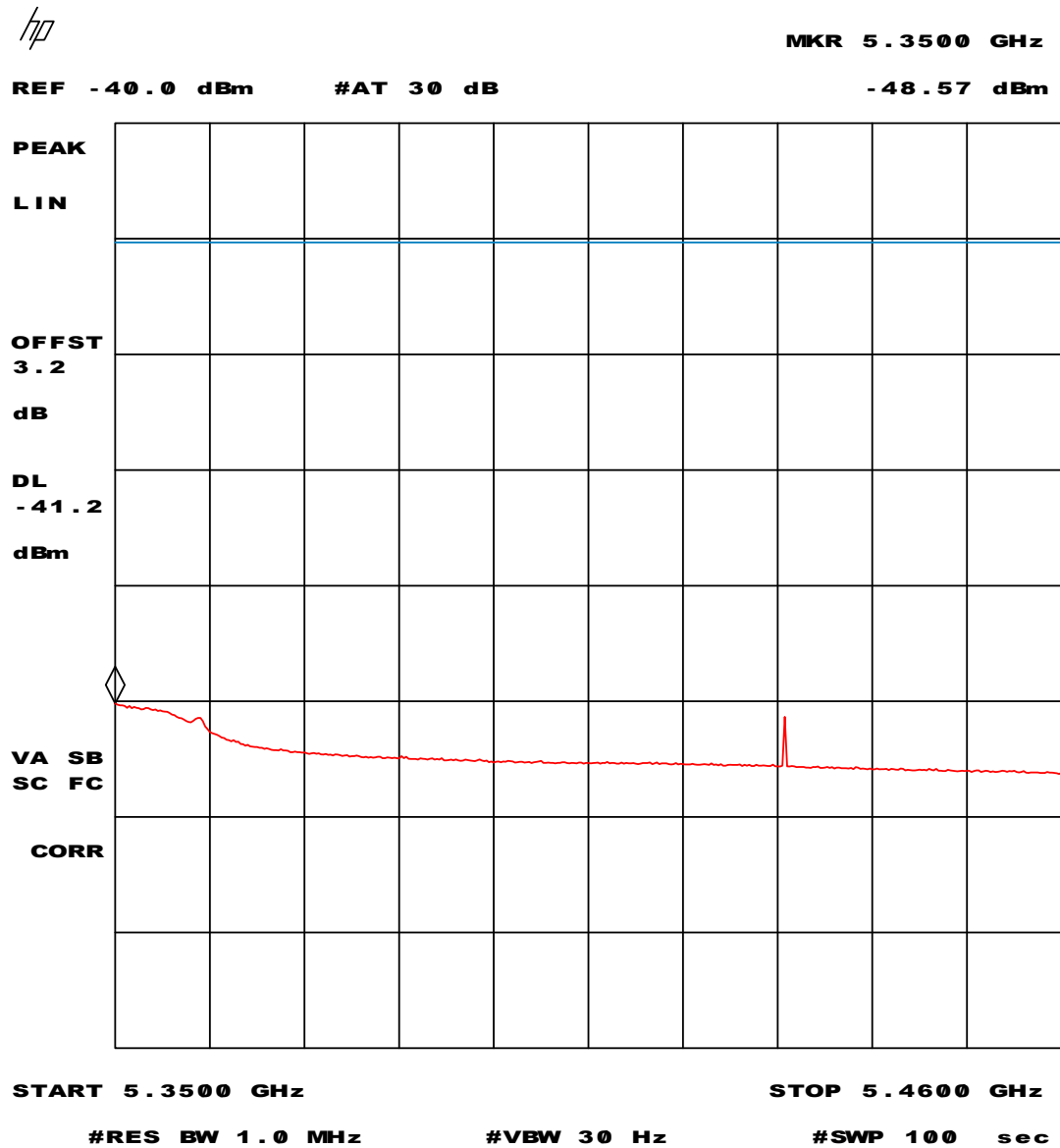
Plot 45 - Average measurement values in the 5.35 – 5.46 GHz restricted band of operation at 0 °C
