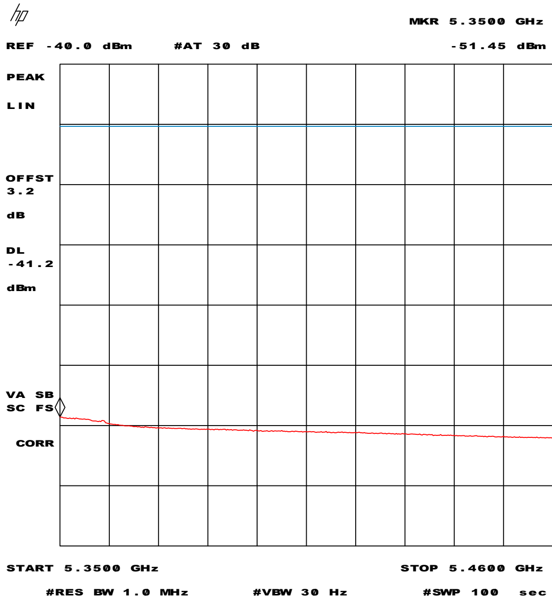
Plot 49 - Average measurement values in the 5.35 – 5.46 GHz restricted band of operation at +50 °C
