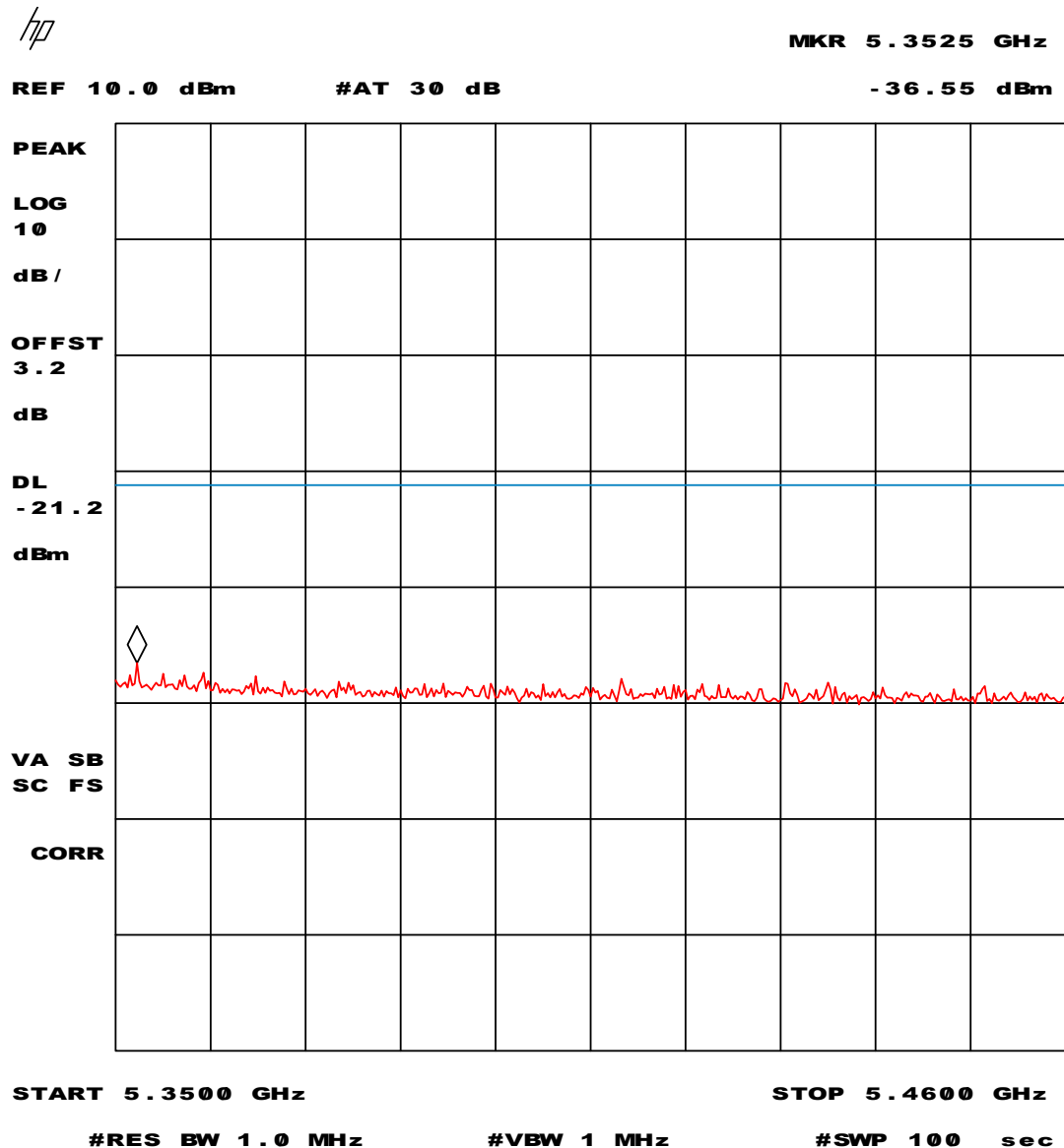
Plot 48 - Peak measurement values in the 5.35 – 5.46 GHz restricted band of operation at +35 °C
