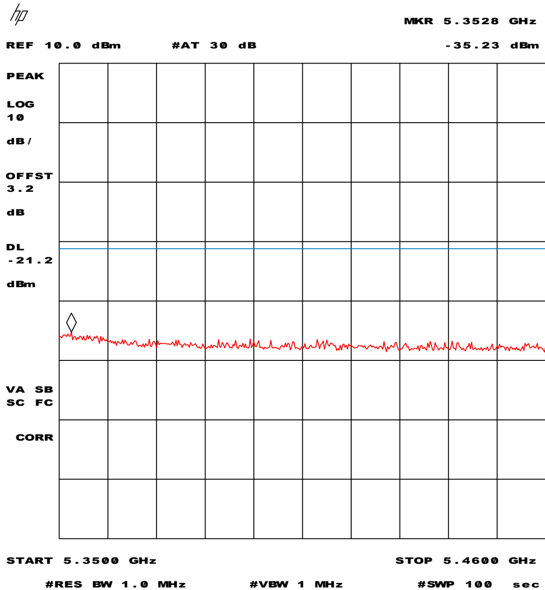
Plot 46 - Peak measurement values in the 5.35 – 5.46 GHz restricted band of operation at 0 °C
