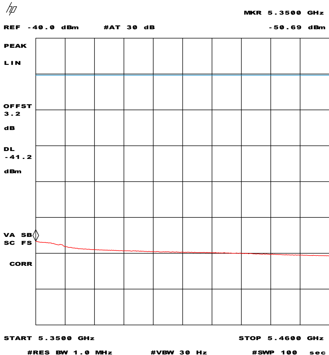
Plot 47 - Average measurement values in the 5.35 – 5.46 GHz restricted band of operation at +35 °C
