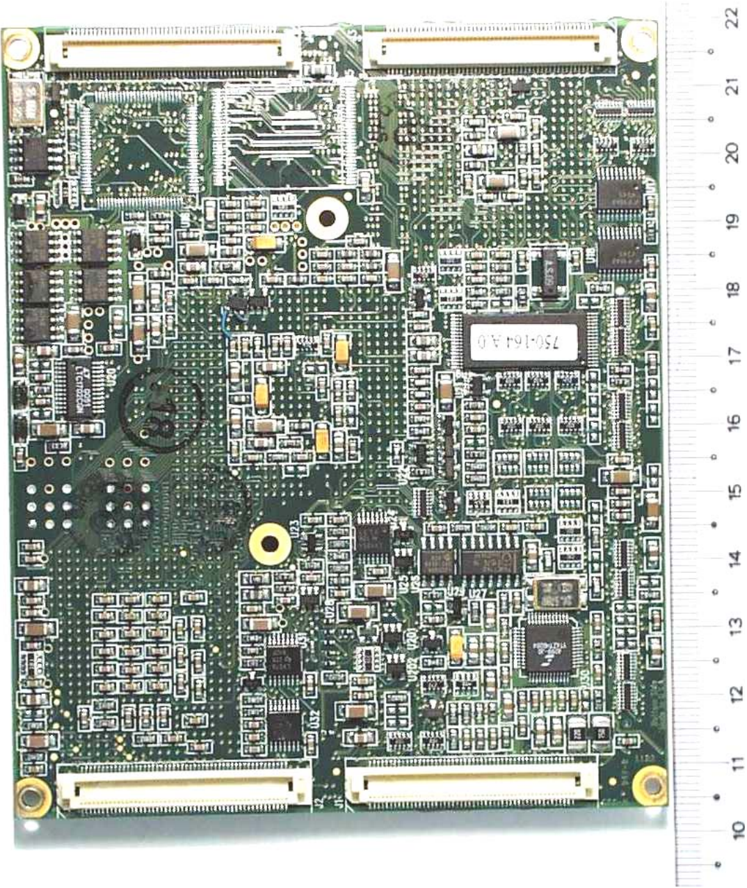
EUT PCB2 – View 1
