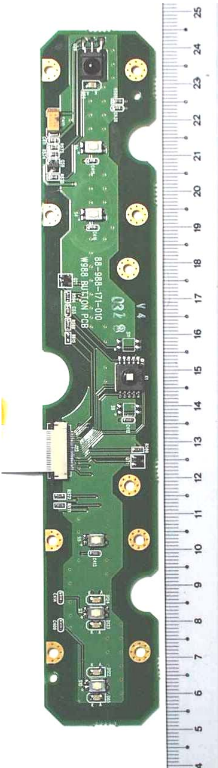
EUT PCB4 – View 2
