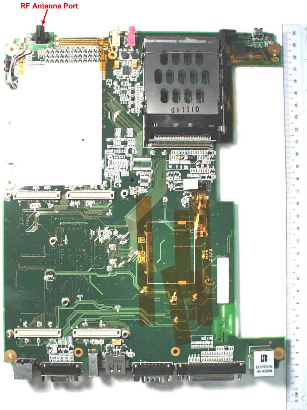
EUT PCB1 – View 1
