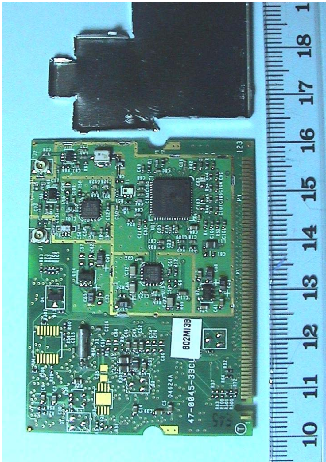
EUT PCB3 – View 3
