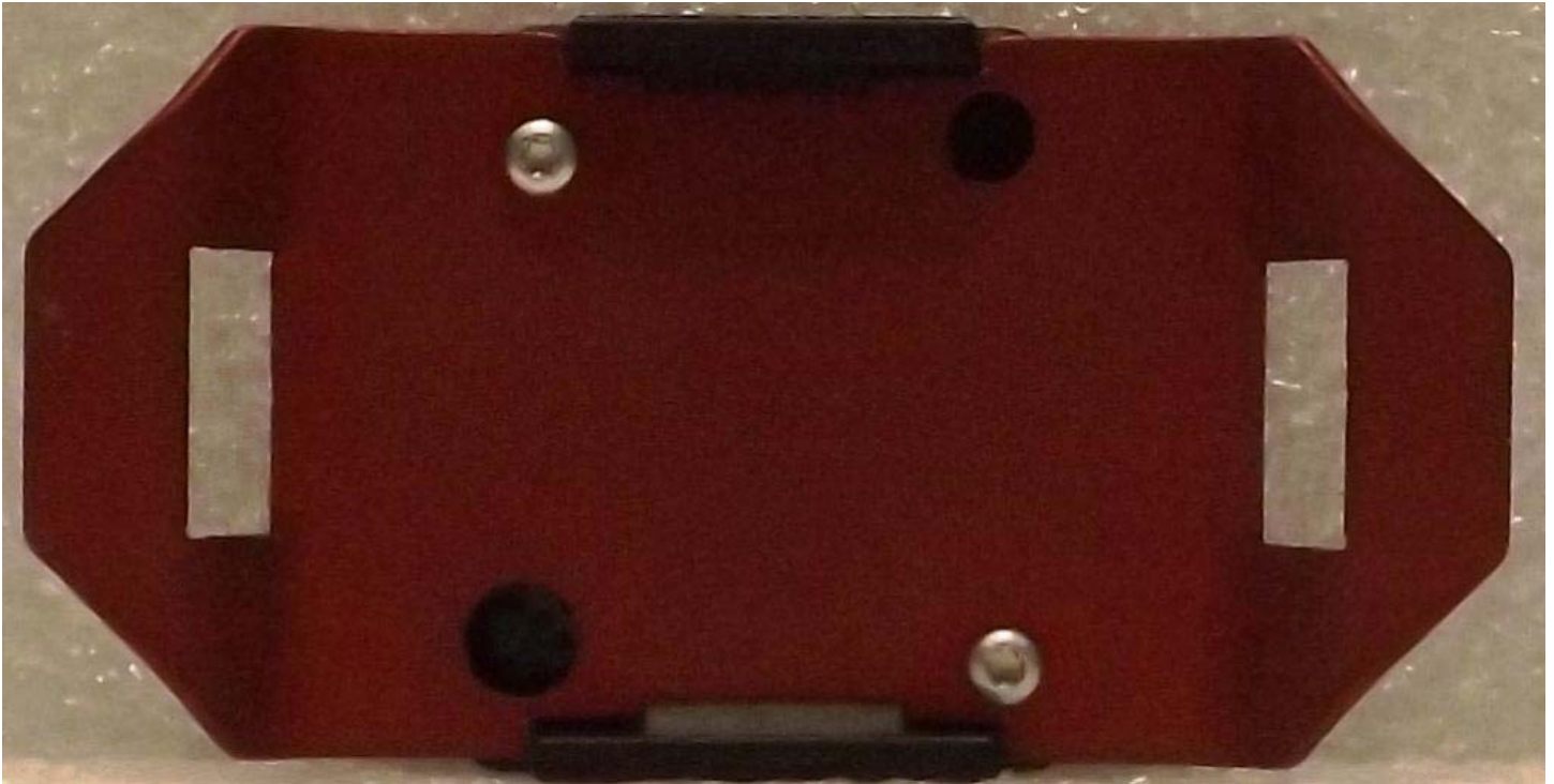
Figure E19.2 – External Photo, TRS-SENSOR-DRY /A – Bottom
