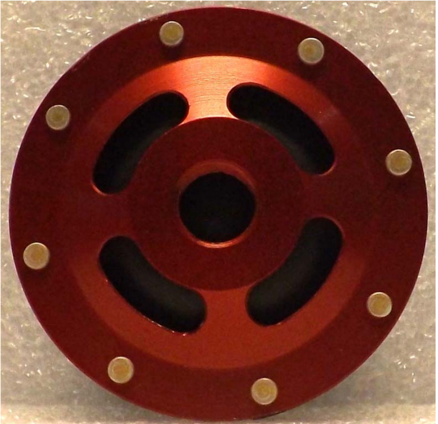
Figure E19.5 – External Photo, TRS-SENSOR-DIA /A – Front
