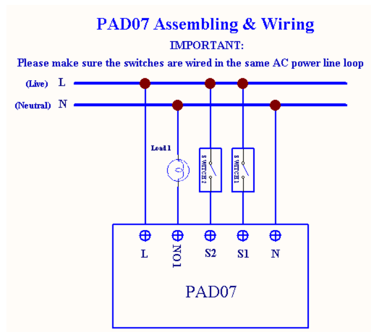
Fig 1. Assembling & Wiring
