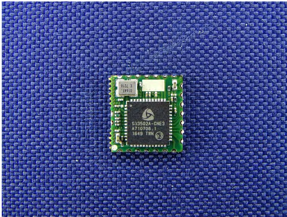
(39) EUT Photo
