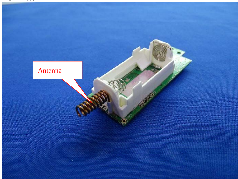
(28) EUT Photo
