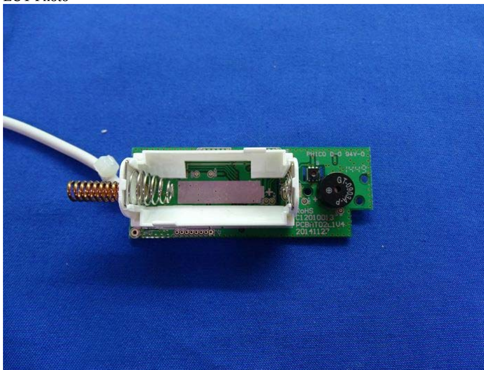
(11) EUT Photo
