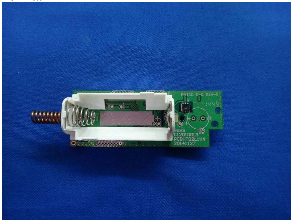
(27) EUT Photo
