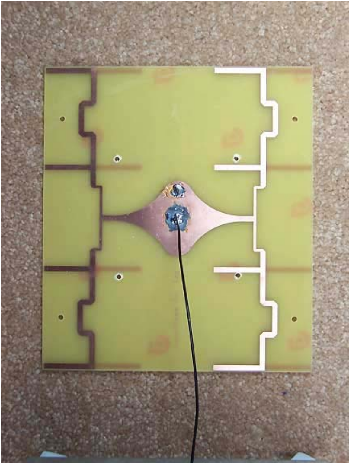
Antenna 24 Directional Back
