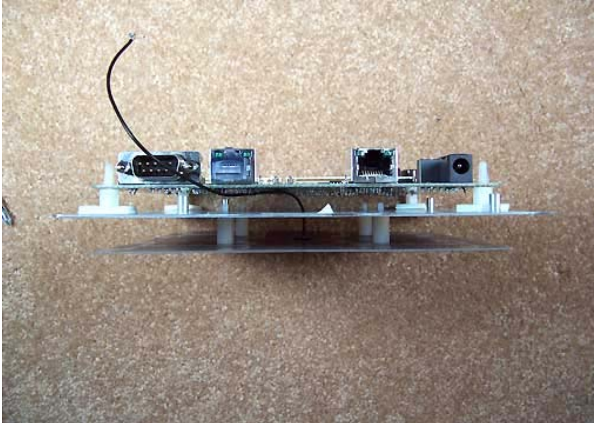
Antenna 5 GHz Directional Side
