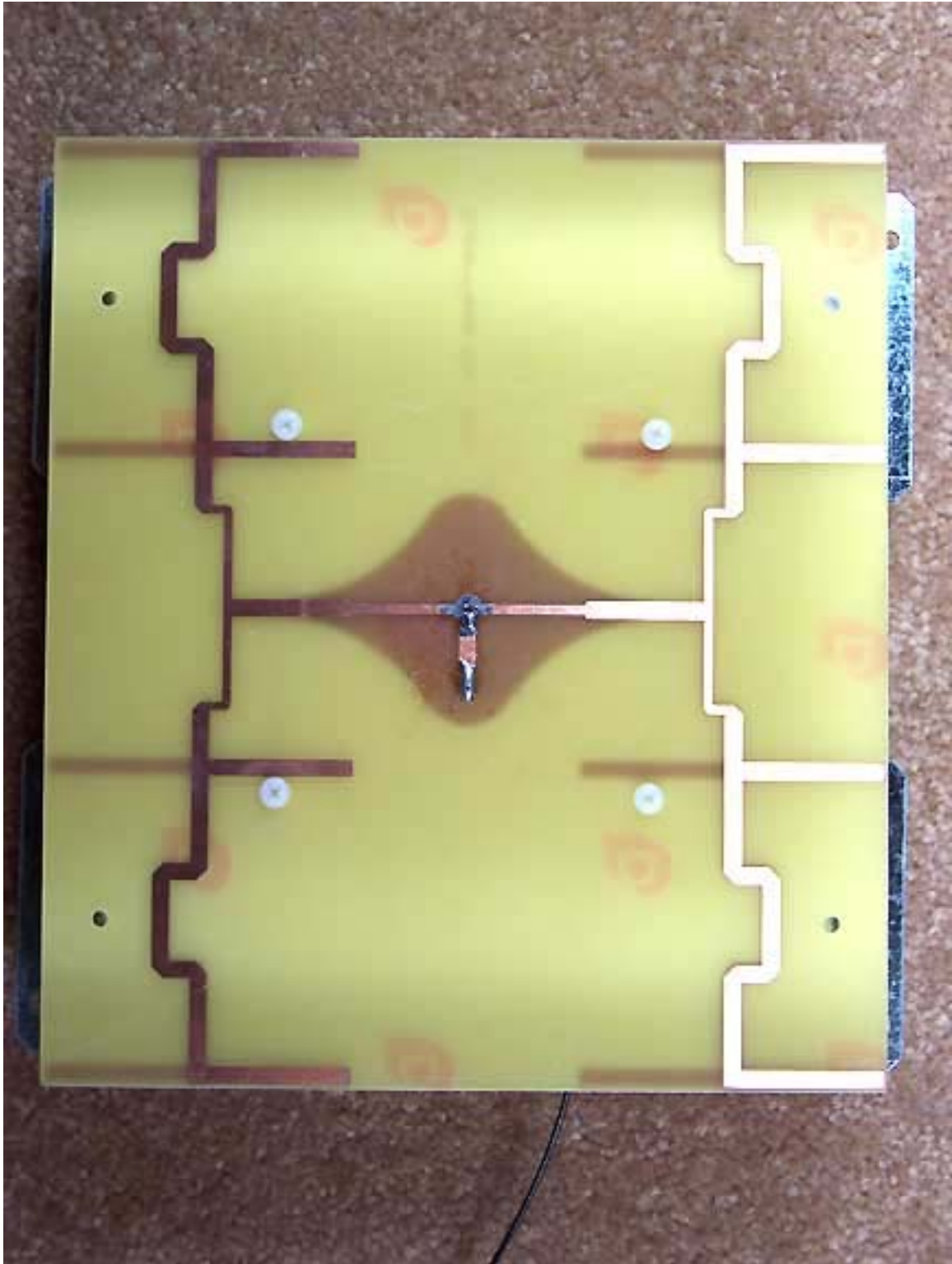
Antenna 24 Directional Front
