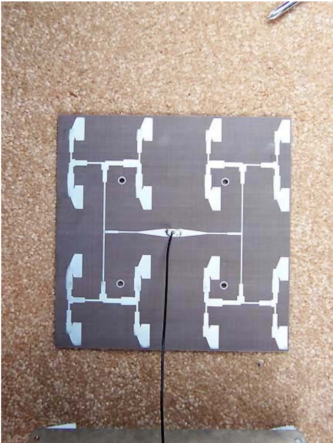
Antenna 5 GHz Directional Back
