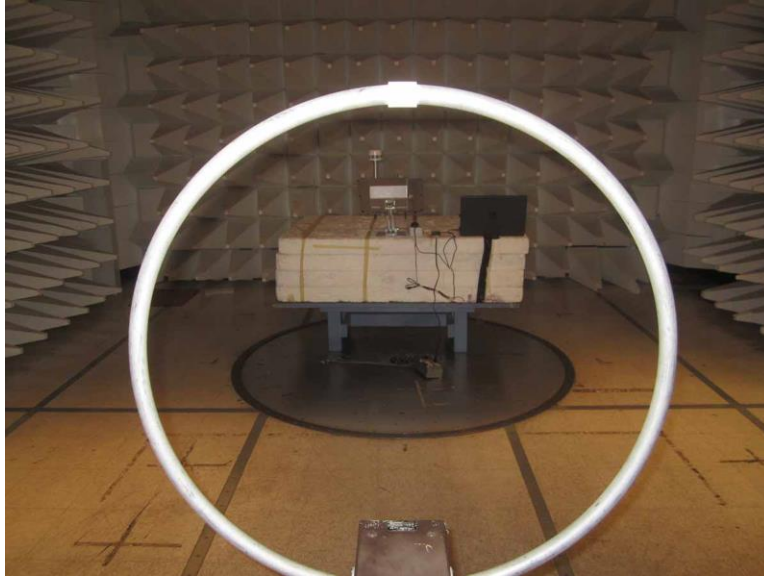
9kHz-30MHz, Parallel
