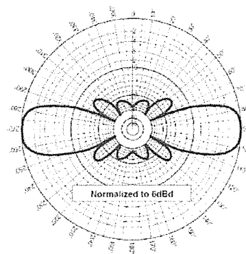
Elevation Pattern (Y, Z or H-plane)
