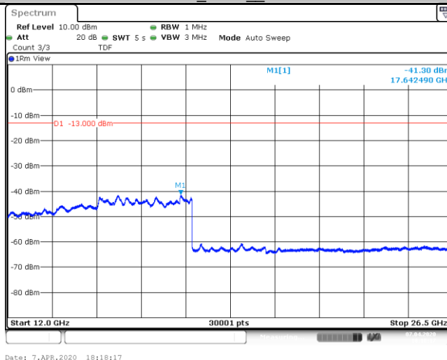
Band71_Stand-Alone_NaN_BPSK_133471_1@11_15kHz_12000_26500_12000-26500MHz@-41.3dBm_-13 PASS
