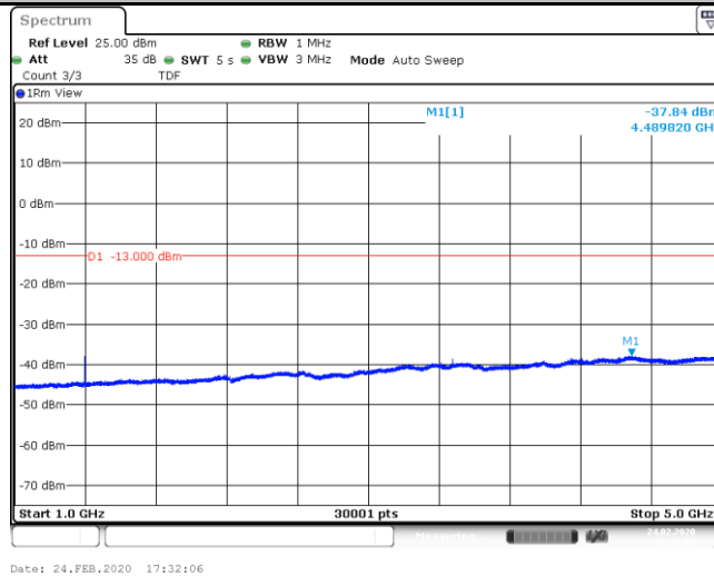
Band85_Stand-Alone_NaN_BPSK_134003_1@0_15kHz_5000_12000_5000~12000MHz@-47.4dBm_-13_PASS__
