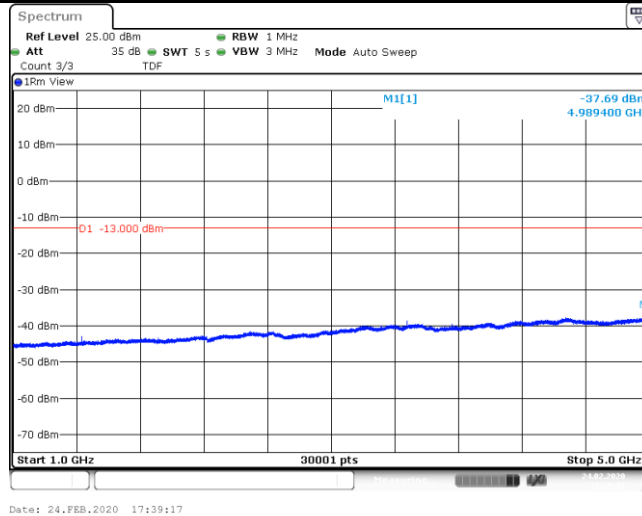
Band85_Stand-Alone_NaN_BPSK_134181_1@0_15kHz_5000_12000_5000~12000MHz@-47.43dBm_-13_PASS__
