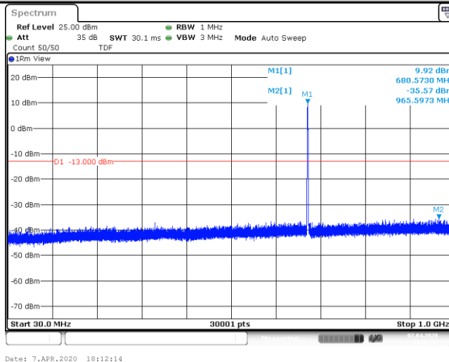
Band71_Stand-Alone_NaN_BPSK_133297_1@11_15kHz_5000_12000_5000~12000MHz@-47.39dBm_-13_ PASS
