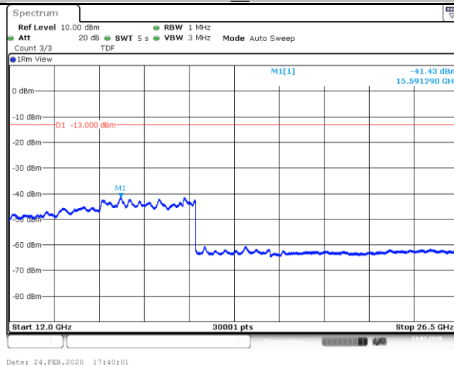
Band85_Stand-Alone_NaN_BPSK_134181_1@0_15kHz_12000_26500_12000~26500MHz@-41.43dBm_-13_PAS S__
