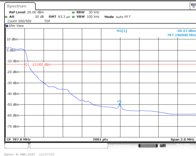
Band13_5MHz_16QAM_23255_1_5_High
