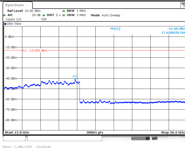
Band13_5MHz_16QAM_23255_1_5_High_12000_26500_-41.6_PASS__
