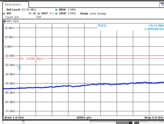
Band12_1.4MHz_QPSK_23017_6_0_Low_1000_5000_-25.41_PASS__
