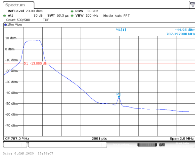
Band13_5MHz_QPSK_23255_1_5_High
