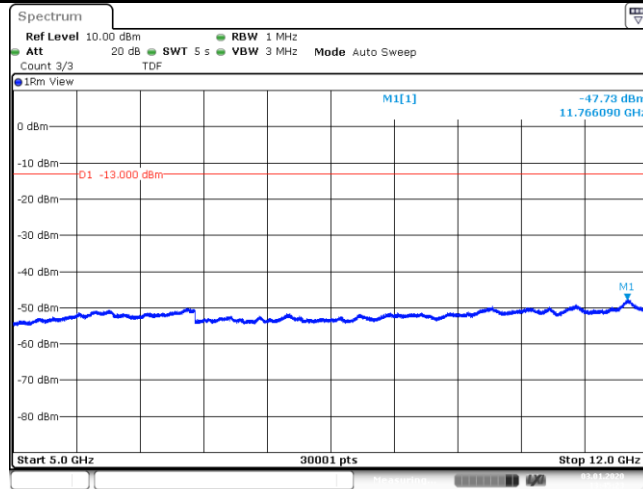
Band12_1.4MHz_QPSK_23017_6_0_Low_5000_12000_-47.73_PASS__
