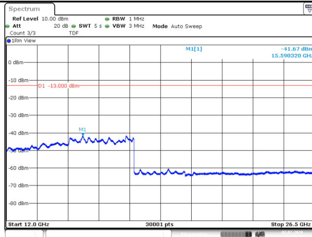
Band12_1.4MHz_QPSK_23017_6_0_Low_12000_26500_-41.67_PASS__
