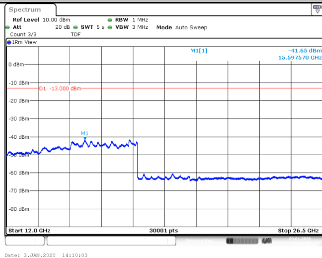
Band13_5MHz_QPSK_23205_1_0_Low_12000_26500_-41.65_PASS__
