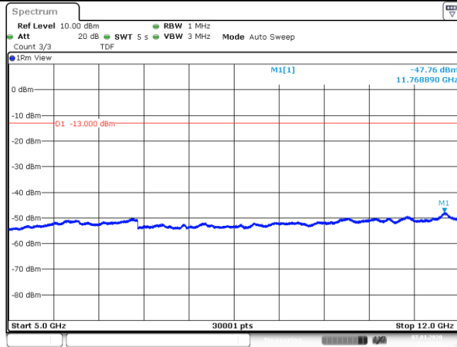
Band26_1.4MHz_QPSK_26797_1_0_Low_5000_12000_-47.76_PASS__
