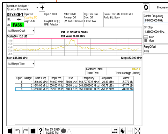
Band5 3MHz QPSK RB1 14 CH20635
