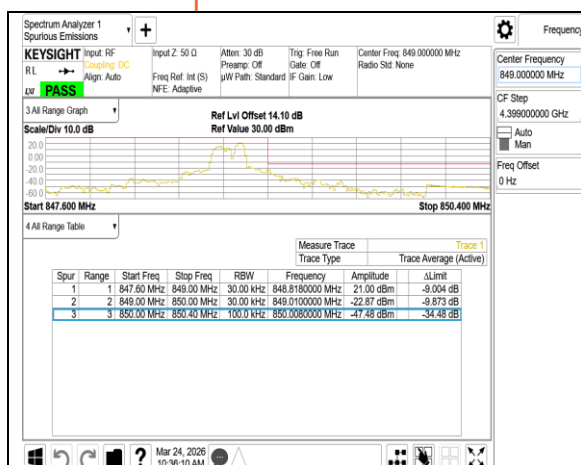
Band26 1.4MHz QPSK RB1 5 CH27033
