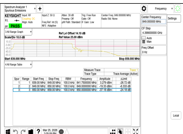
Band26 10MHz QPSK RB50 0 CH26990
