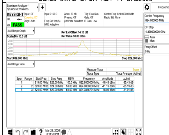
Band5 5MHz QPSK RB1 0 CH20425
