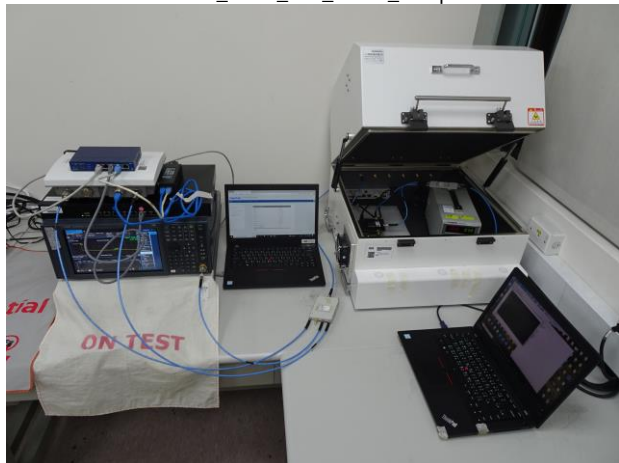
FCC_96.47_NR_CBSD_Setup
