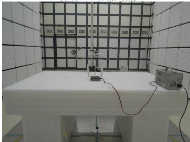
FCC_96.47_LTE_CBSD_Setup
