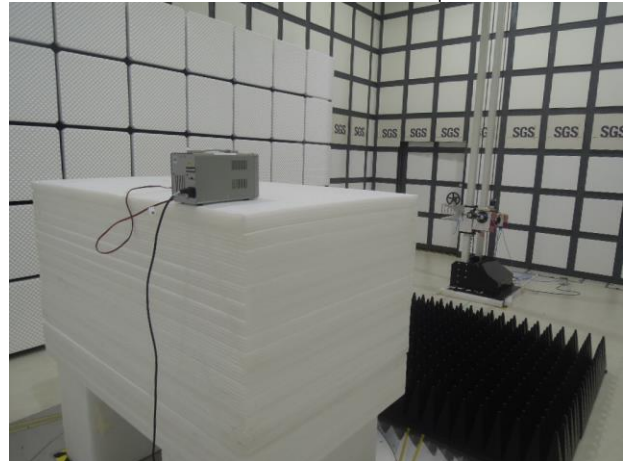
FCC_96_NR_Radiated_Setup
