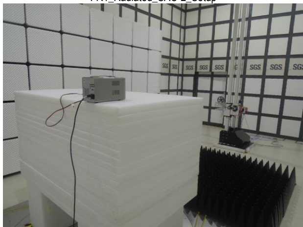
FR1_Radiated_SAC-2_Setup
