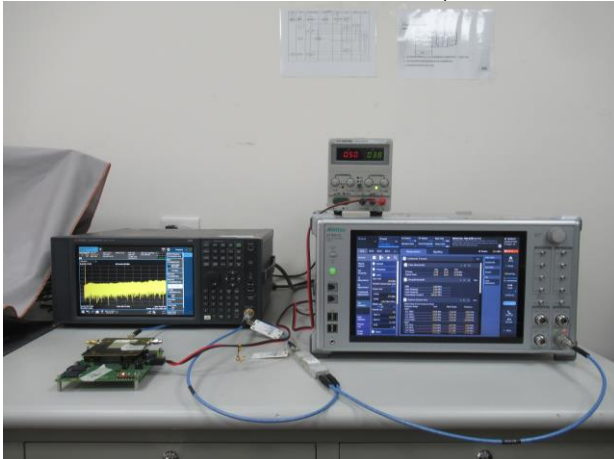
FCC_96_LTE_Conducted_Setup
