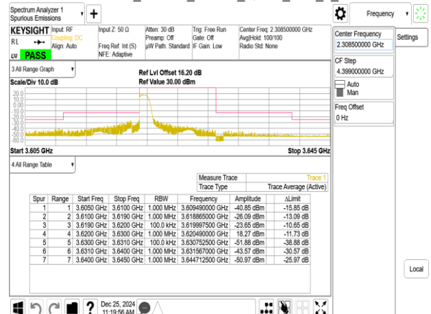
Emission Mask_Band48_10MHz_QPSK_RB1_0_CH56690
