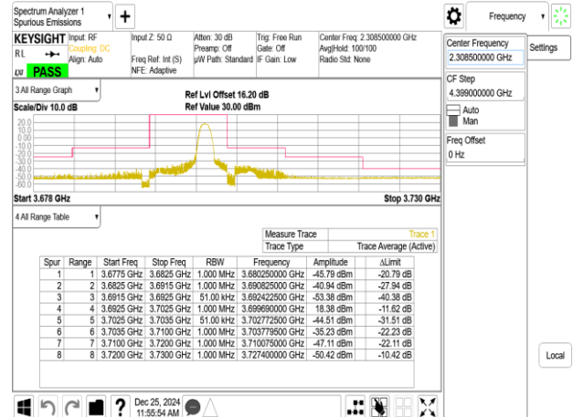
Emission Mask_Band48_5MHz_QPSK_RB1_24_CH56715
