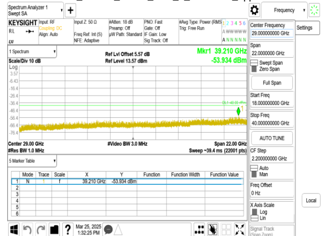
Band48_20MHz_QPSK_RB1_0_CH56640_upper 18G
