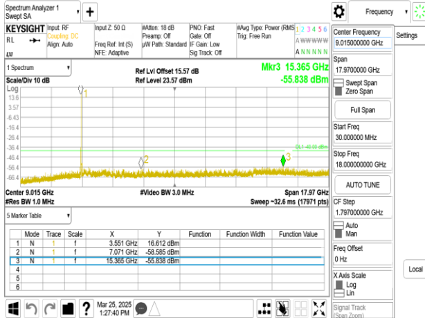
Band48_20MHz_QPSK_RB1_0_CH55340_upper 18G
