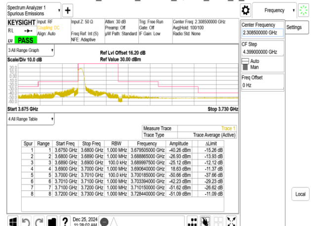
Emission Mask_Band48_10MHz_QPSK_RB1_0_CH56690
