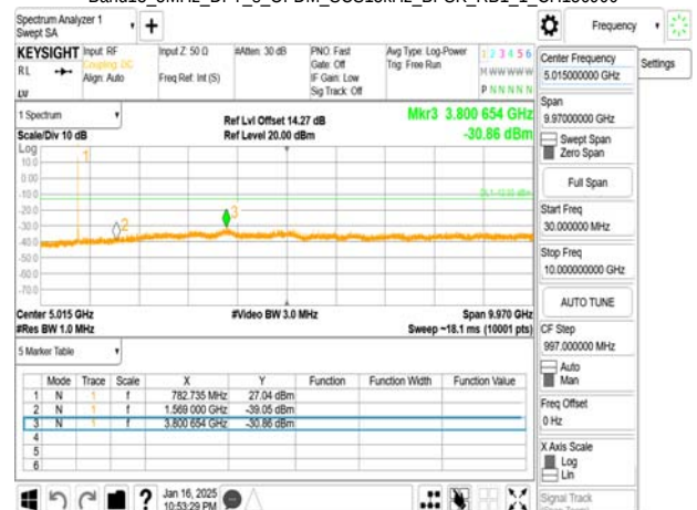
Band13 5MHz DFT s OFDM_SCS15kHz_BPSK_RB1_1_CH156900
