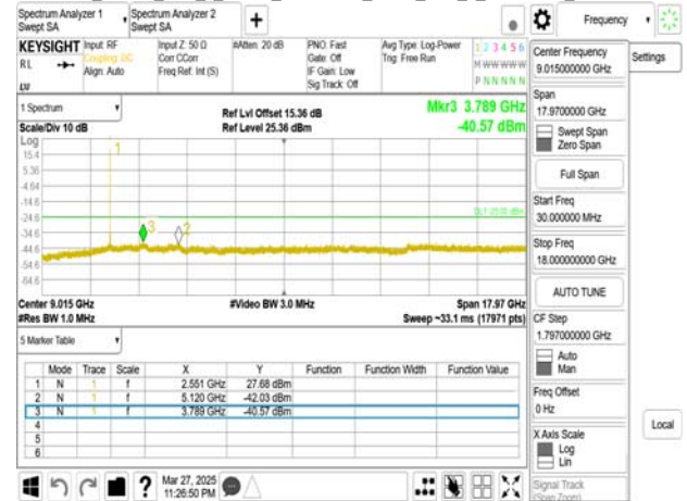
Band7 20MHz DFT s OFDM_SCS15kHz_BPSK_RB1_1_CH512000upper 18G
