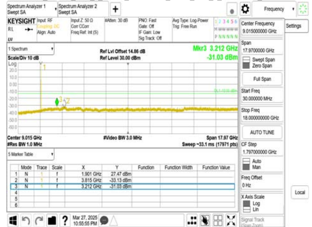
Band25_15MHz_DFT_s_OFDM_SCS15kHz_BPSK_RB1_1_CH381500upper 18G
