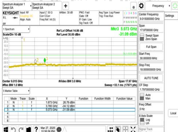
Band25 20MHz DFT s OFDM_SCS15kHz_BPSK_RB1_1_CH376500upper 18G
