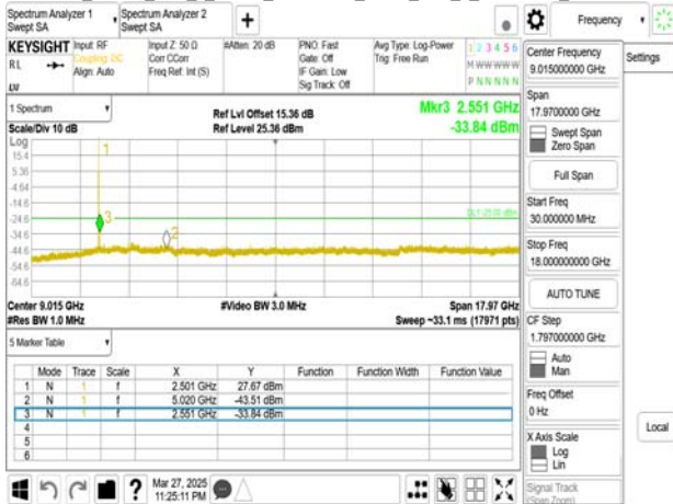
Band7 20MHz DFT s OFDM_SCS15kHz_BPSK_RB1_1_CH502000upper 18G
