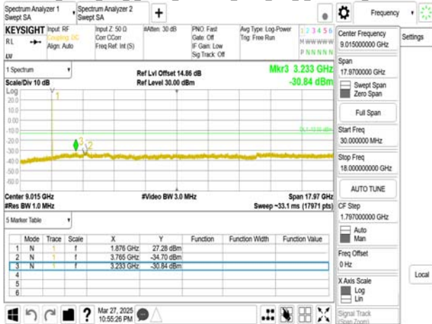
Band25_15MHz_DFT_s_OFDM_SCS15kHz_BPSK_RB1_1_CH376500upper 18G
