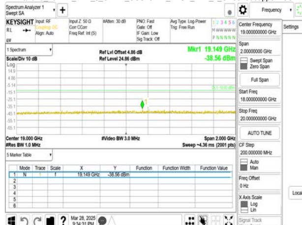
Band26-Part90s 5MHz DFT s OFDM_SCS15kHz_BPSK_RB1_1_CH163300
