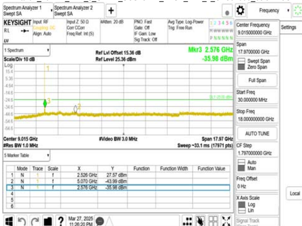
Band7 20MHz DFT s OFDM_SCS15kHz_BPSK_RB1_1_CH507000_below 18G
