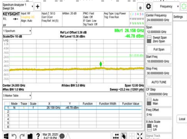
Band38_20MHz_DFT_s_OFDM_SCS30kHz_BPSK_RB1_1_CH519000upper 18G
