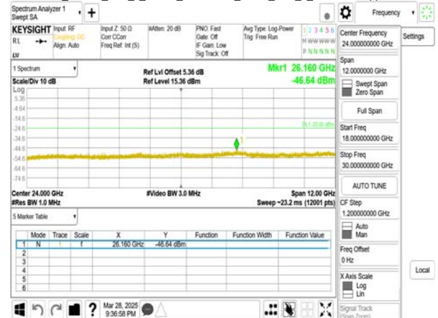
Band7_10MHz_DFT_s_OFDM_SCS15kHz_BPSK_RB1_1_CH513000upper 18G
