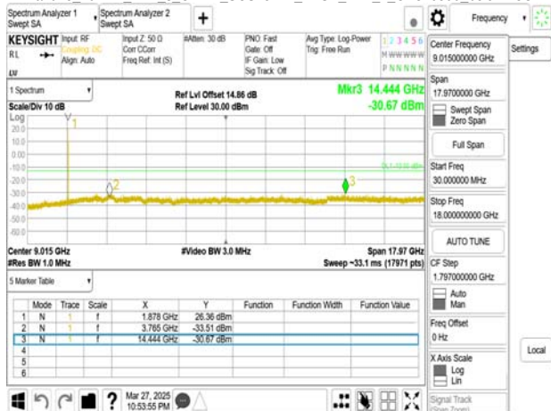
Band25_10MHz_DFT_s_OFDM_SCS15kHz_BPSK_RB1_1_CH376500upper 18G
