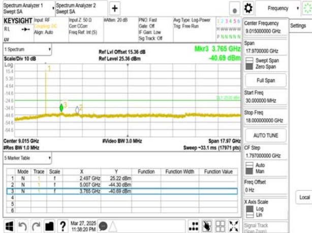
Band41 15MHz DFT s OFDM_SCS30kHz_BPSK_RB1_1_CH500700upper 18G
