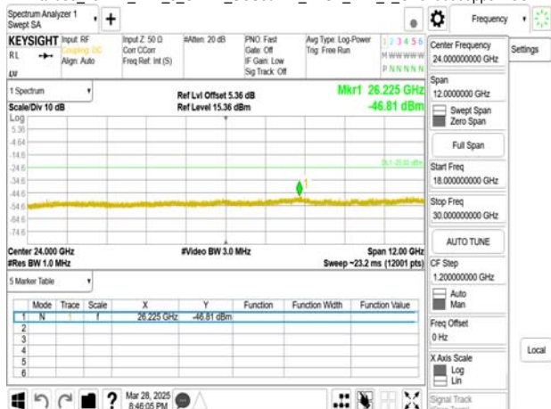
Band38_15MHz_DFT_s_OFDM_SCS30kHz_BPSK_RB1_1_CH519000upper 18G
