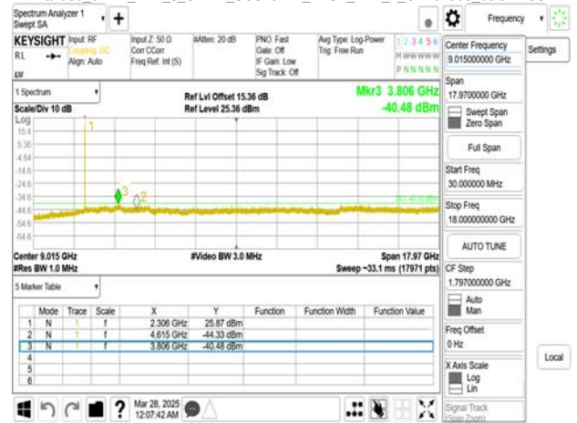
Band30 5MHz DFT s OFDM_SCS15kHz BPSK RB1 1 CH461500upper 18G
