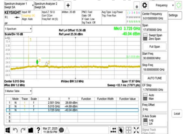
Band41 15MHz DFT s OFDM_SCS30kHz_BPSK_RB1_1_CH501504upper 18G
