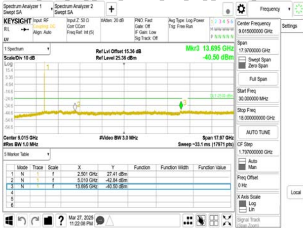
Band7_10MHz_DFT_s_OFDM_SCS15kHz_BPSK_RB1_1_CH501000upper 18G
