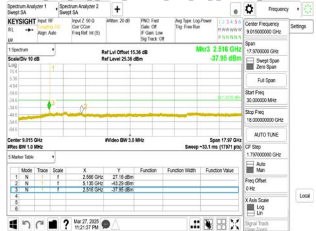
Band7_5MHz_DFT_s_OFDM_SCS15kHz_BPSK_RB1_1_CH513500upper 18G
