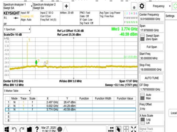
Band41_10MHz_DFT_s_OFDM_SCS30kHz_BPSK_RB1_1_CH500202 below 18G
