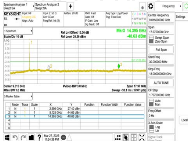
Band7_15MHz_DFT_s_OFDM_SCS15kHz_BPSK_RB1_1_CH512500upper 18G
