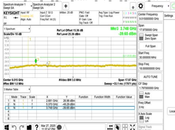
Band41_10MHz_DFT_s_OFDM_SCS30kHz_BPSK_RB1_1_CH537000 below 18G
