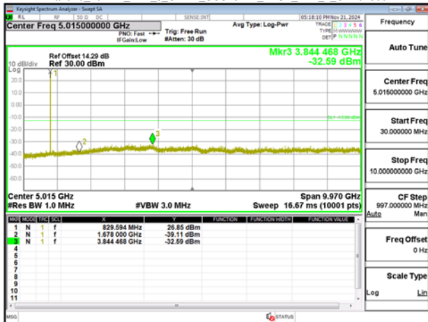
Band26 20MHz DFT s OFDM_SCS15kHz BPSK RB1 1 CH167800
