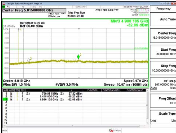
Band12 15MHz DFT s OFDM_SCS15kHz_BPSK_RB1_1_CH141700
