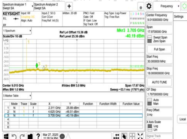
Band30 5MHz_DFT_s_OFDM_SCS15kHz_BPSK_RB1_1_CH462500upper 18G
