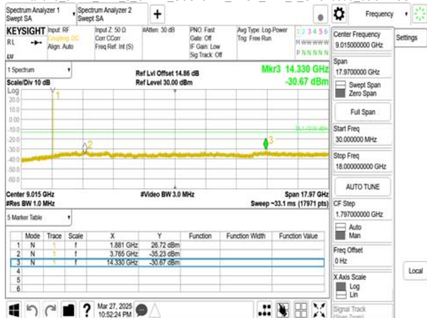
Band25 5MHz_DFT_s_OFDM_SCS15kHz_BPSK_RB1_1_CH376500upper 18G
