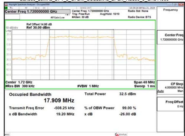
Band66 20MHz DFT s OFDM SCS15kHz BPSK RB100 0 CH344000
