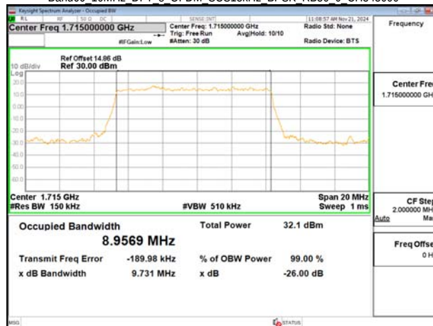
Band66 10MHz DFT s OFDM SCS15kHz BPSK RB50 0 CH343000
