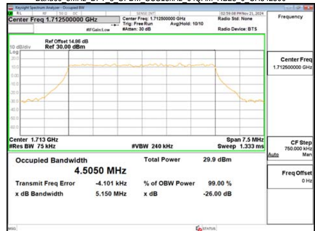
Band66 5MHz DFT s OFDM SCS15kHz 64QAM RB25 0 CH342500
