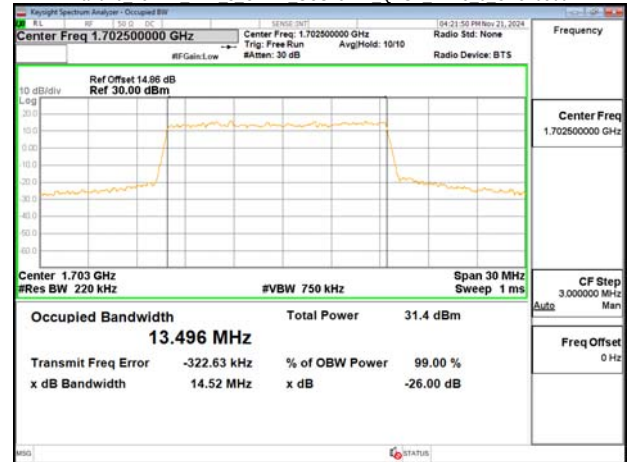
Band70 15MHz DFT s OFDM SCS15kHz 16QAM RB75 0 CH340500
