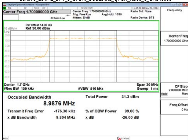
Band70 10MHz DFT s OFDM SCS15kHz QPSK RB50 0 CH340000
