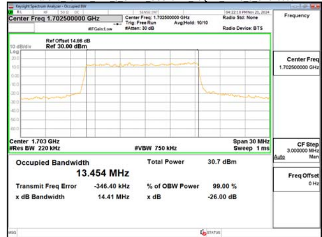
Band70 15MHz DFT s OFDM SCS15kHz 64QAM RB75 0 CH340500
