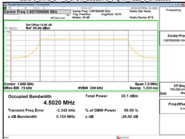
Band70 5MHz DFT s OFDM SCS15kHz 64QAM RB25 0 CH339500
