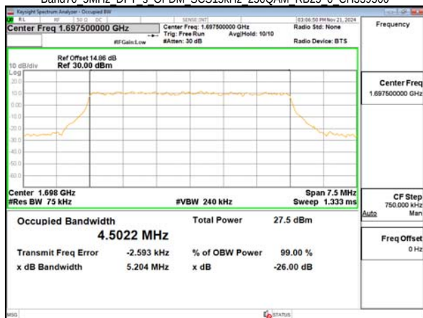
Band70 5MHz DFT s OFDM SCS15kHz 256QAM RB25 0 CH393500
