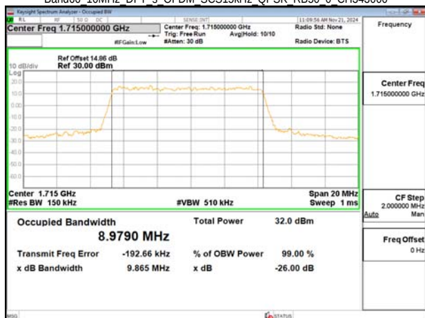
Band66 10MHz DFT s OFDM SCS15kHz QPSK RB50 0 CH343000
