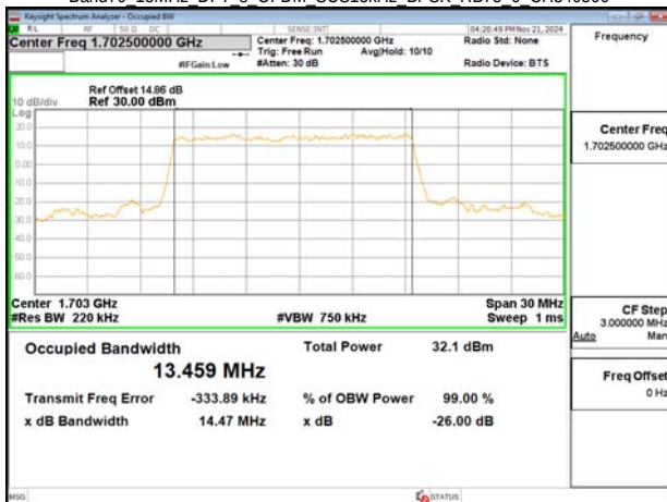
Band70 15MHz DFT s OFDM SCS15kHz BPSK RB75 0 CH340500
