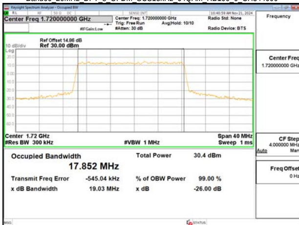
Band66 20MHz DFT s OFDM SCS15kHz 64QAM RB100 0 CH344000
