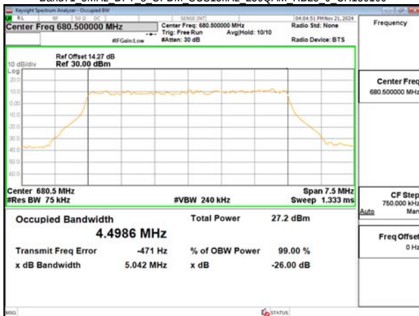
Band71 5MHz DFT s OFDM SCS15kHz 256QAM RB25 0 CH136100
