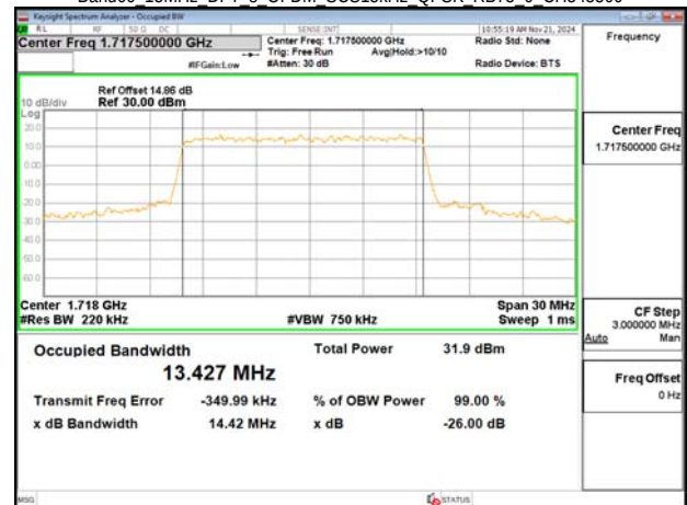
Band66 15MHz DFT s OFDM SCS15kHz QPSK RB75 0 CH343500
