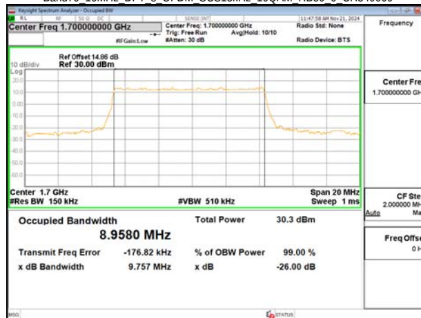
Band70 10MHz DFT s OFDM SCS15kHz 16QAM RB50 0 CH340000
