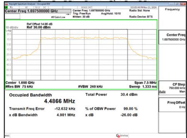
Band70 5MHz DFT s OFDM SCS15kHz QPSK RB25 0 CH339500
