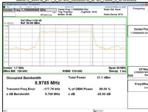
Band70 10MHz DFT s OFDM SCS15kHz BPSK RB50 0 CH340000
