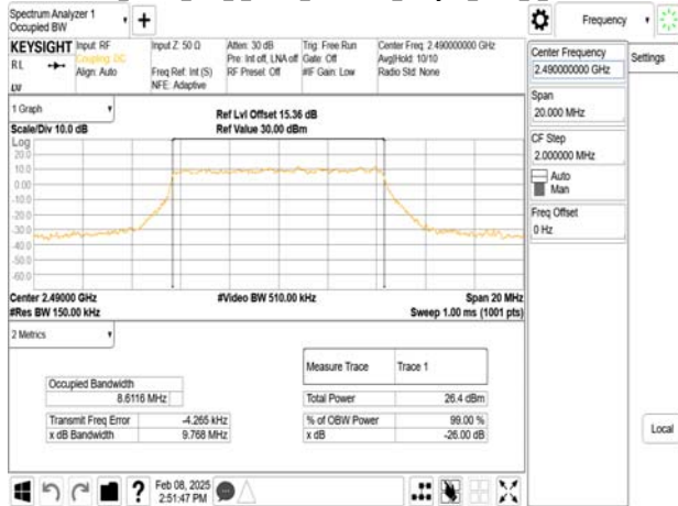
Band53 10MHz DFT s OFDM_SCS30kHz_256QAM_RB24_0_CH498000
