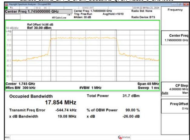
Band66 20MHz DFT s OFDM SCS15kHz QPSK RB100 0 CH349000
