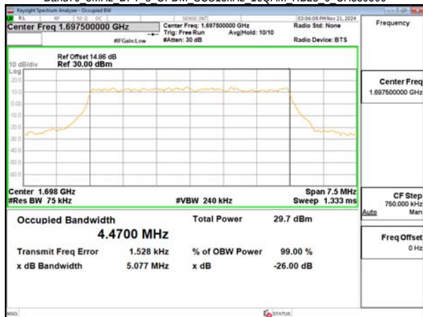
Band70 5MHz DFT s OFDM SCS15kHz 16QAM RB25 0 CH339500
