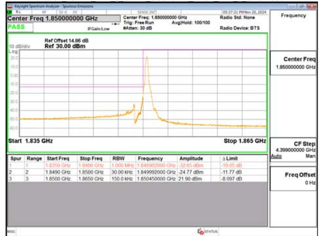
Band2 15MHz DFT s OFDM SCS15kHz BPSK RB75 0 CH371500
