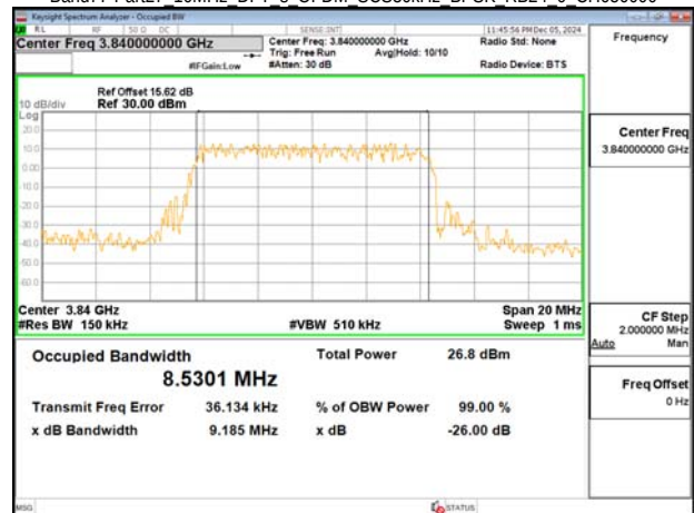
Band77-Part27 10MHz DFT s OFDM SCS30kHz BPSK RB24 0 CH656000
