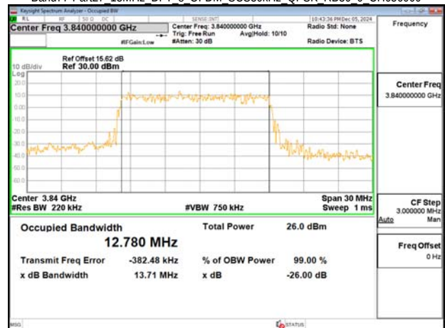
Band77-Part27 15MHz DFT s OFDM SCS30kHz QPSK RB36 0 CH656000
