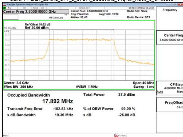
Band77-Part27 20MHz DFT s OFDM SCS30kHz 64QAM RB50 0 CH633334
