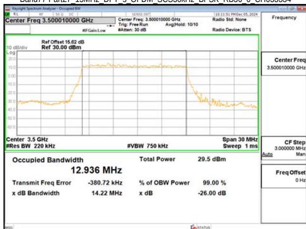
Band77-Part27 15MHz DFT s OFDM SCS30kHz BPSK RB36 0 CH633334
