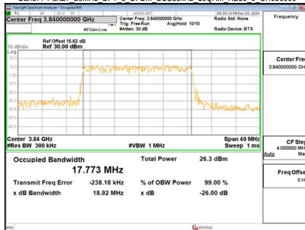
Band77-Part27 20MHz DFT s OFDM SCS30kHz 16QAM RB50 0 CH656000
