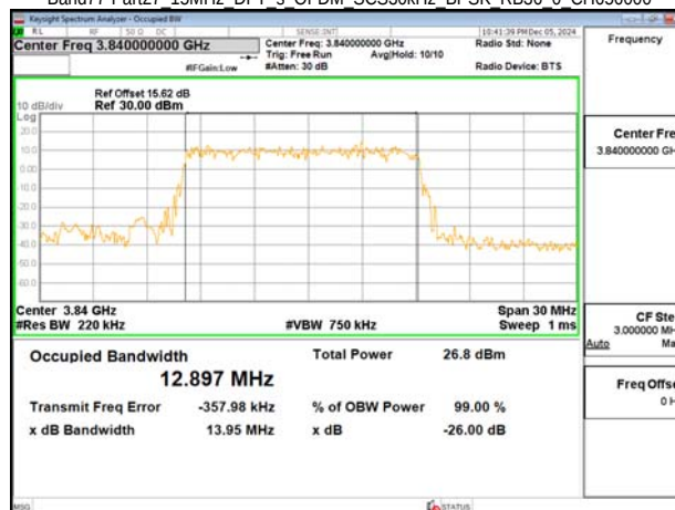
Band77-Part27 15MHz DFT s OFDM SCS30kHz BPSK RB36 0 CH656000
