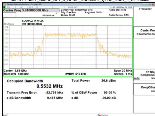
Band77-Part27 10MHz DFT s OFDM SCS30kHz QPSK RB24 0 CH656000
